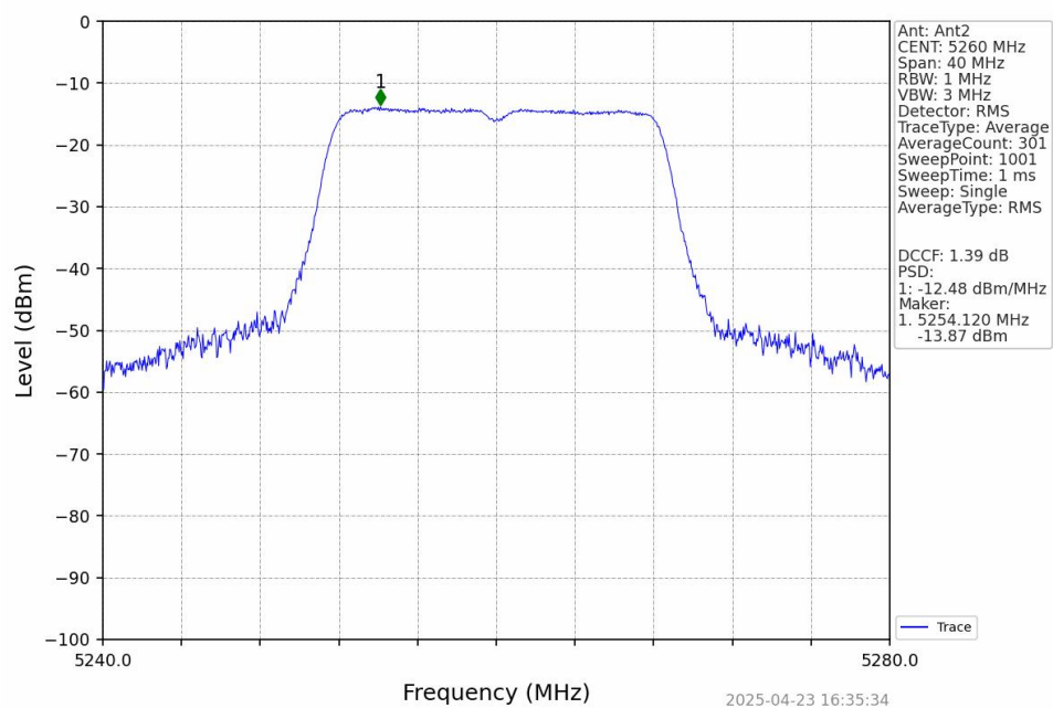
802.11a_LCH_5260MHz_Ant2_NTNV
