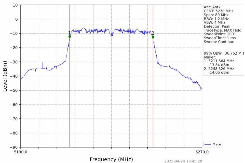
802.11ac(VHT40)_HCH_5230MHz_Ant2_NTNV
