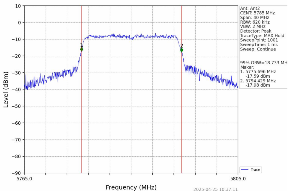
802.11ac(VHT20)_MCH_5785MHz_Ant2_NTNV
