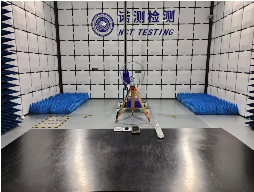
Setup Photo FCC ID: 2A4WMABC-A151
