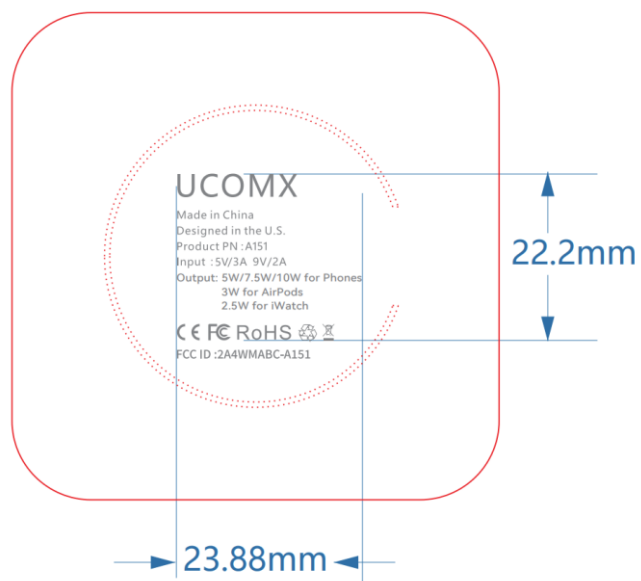
Label
