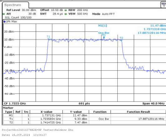
99%OBW Band 4 20MHz/1732.5/Mid 16QAM 100@0
