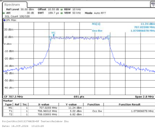
99%OBW Band 12 1.4MHz/707.5/Mid 16QAM 6@0
