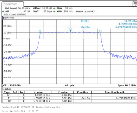
99%OBW Band 4 5MHz/1732.5/Mid 16QAM 25@0
