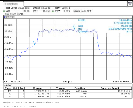
26%OBW Band 4 20MHz/1732.5/Mid 16QAM 100@0
