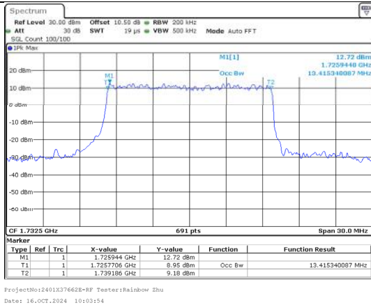
99%OBW Band 4 15MHz/1732.5/Mid 16QAM 75@0
