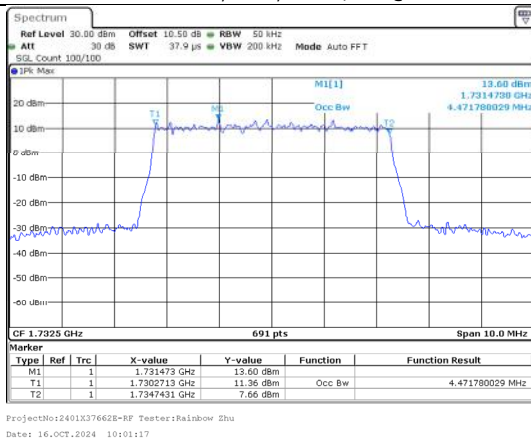
99%OBW Band 4 5MHz/1732.5/Mid QPSK 25@0
