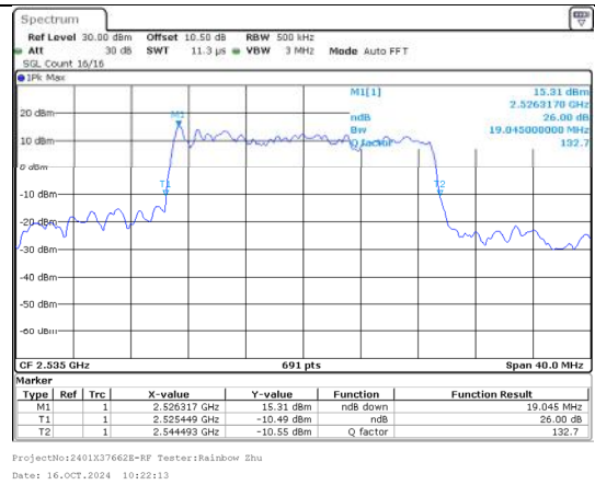
26%OBW Band 7 20MHz/2535.0/Mid 16QAM 100@0
