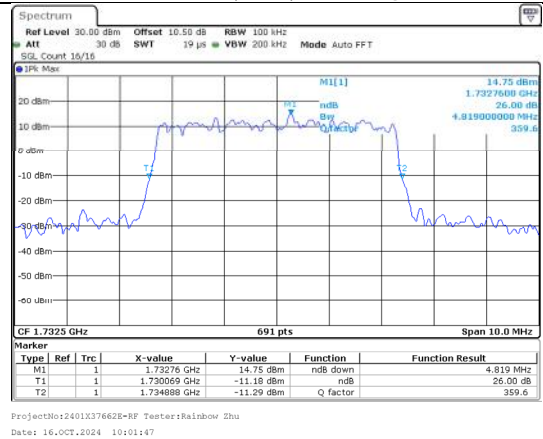
26%OBW Band 4 5MHz/1732.5/Mid 16QAM 25@0
