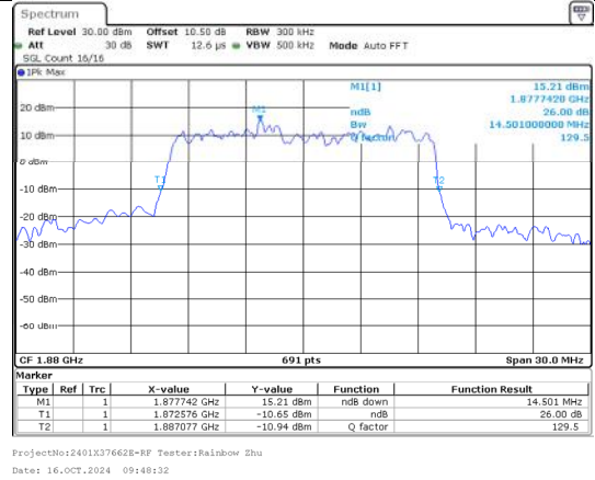
26%OBW Band 2 15MHz/1880.0/Mid 16QAM 75@0
