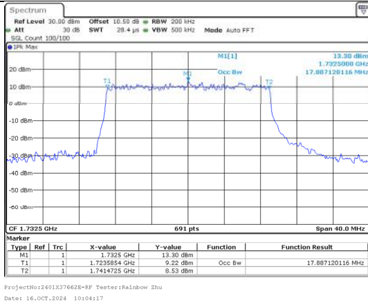
99%OBW Band 4 20MHz/1732.5/Mid QPSK 100@0
