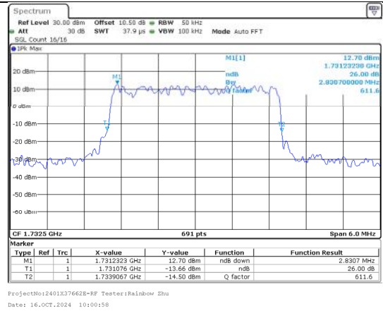
26%OBW Band 4 3MHz/1732.5/Mid 16QAM 15@0
