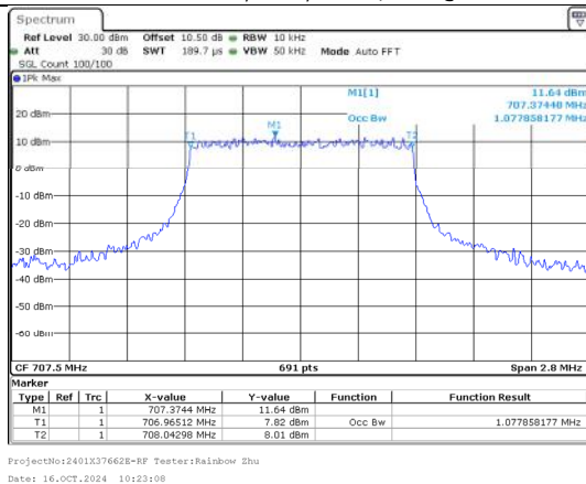
99%OBW Band 12 1.4MHz/707.5/Mid QPSK 6@0
