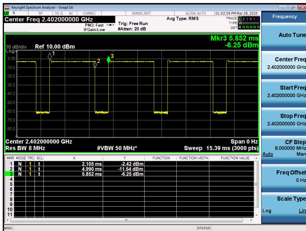
EDR-π /4-DQPSK-ANT1-2402
