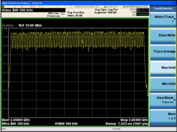
8DPSK Modulation
