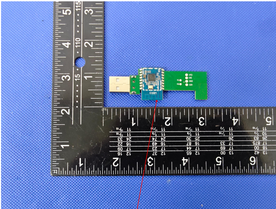
WIFI ANT
