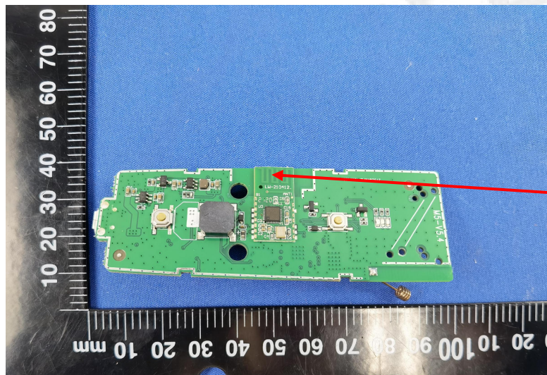
Bluetooth Antenna
