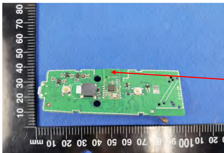
Bluetooth Antenna
