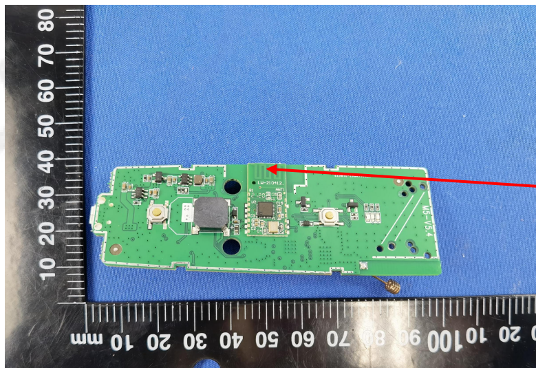
Bluetooth Antenna
