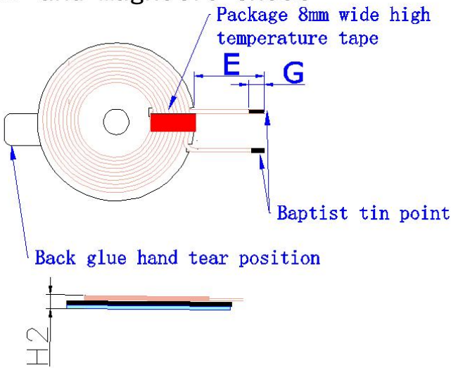
Figure 3. Combination of coil and magnetic sheet
