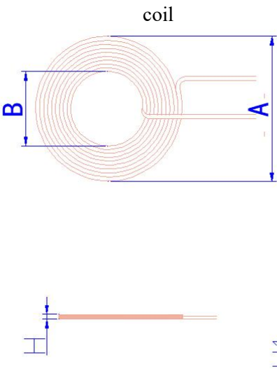
Figure 1. Coil
