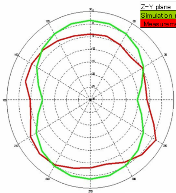
Z-Y Plane
