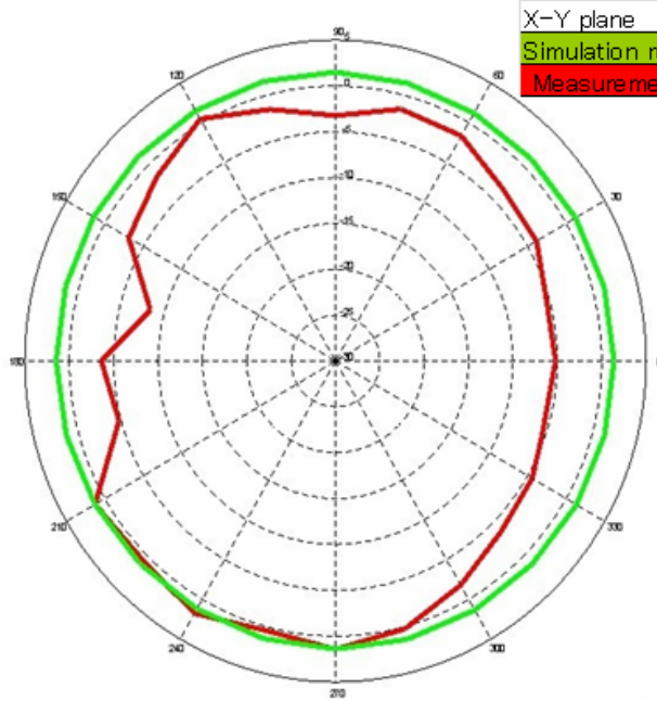
X-Y Plane
