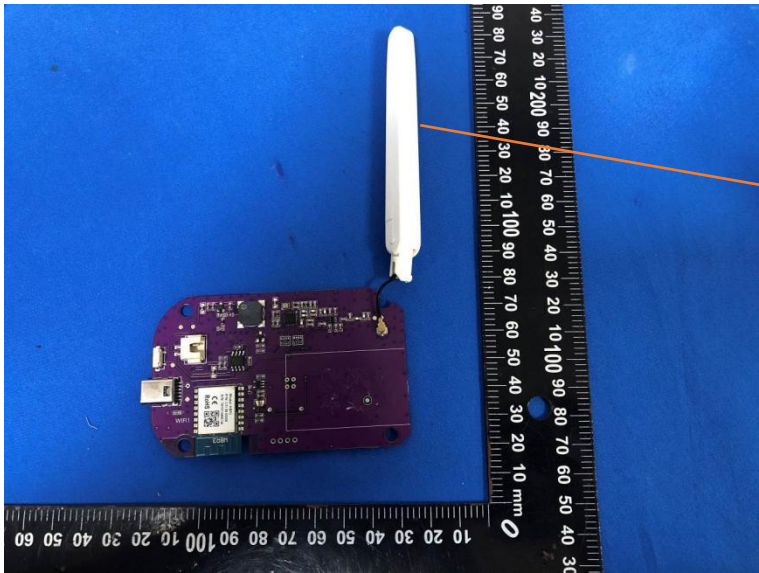
433MHz ANT
