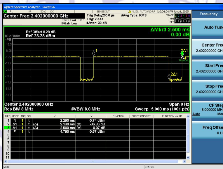
Duty_Cycle_NVNT_ANT1_1Mbps_2402
