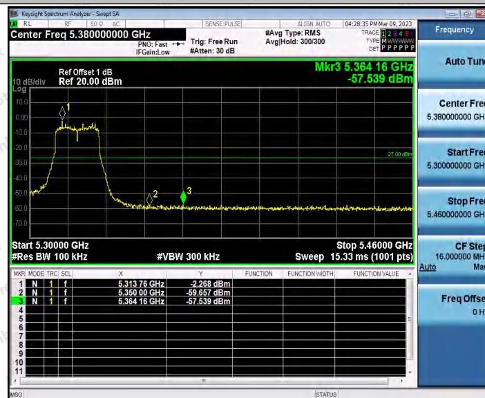
11N20SISO_Ant1_High_5320
