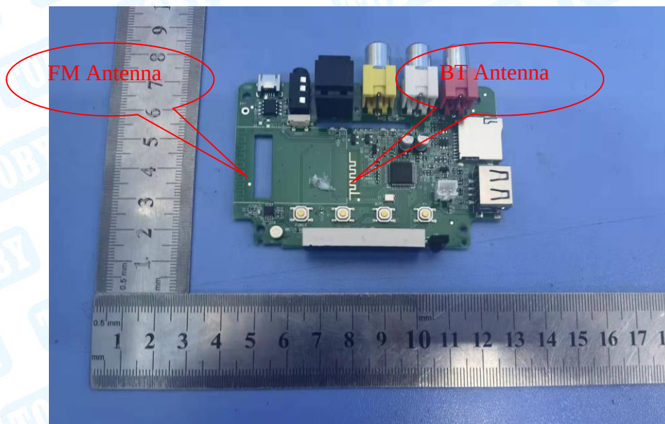
Photo 9 Appearance of PCB
