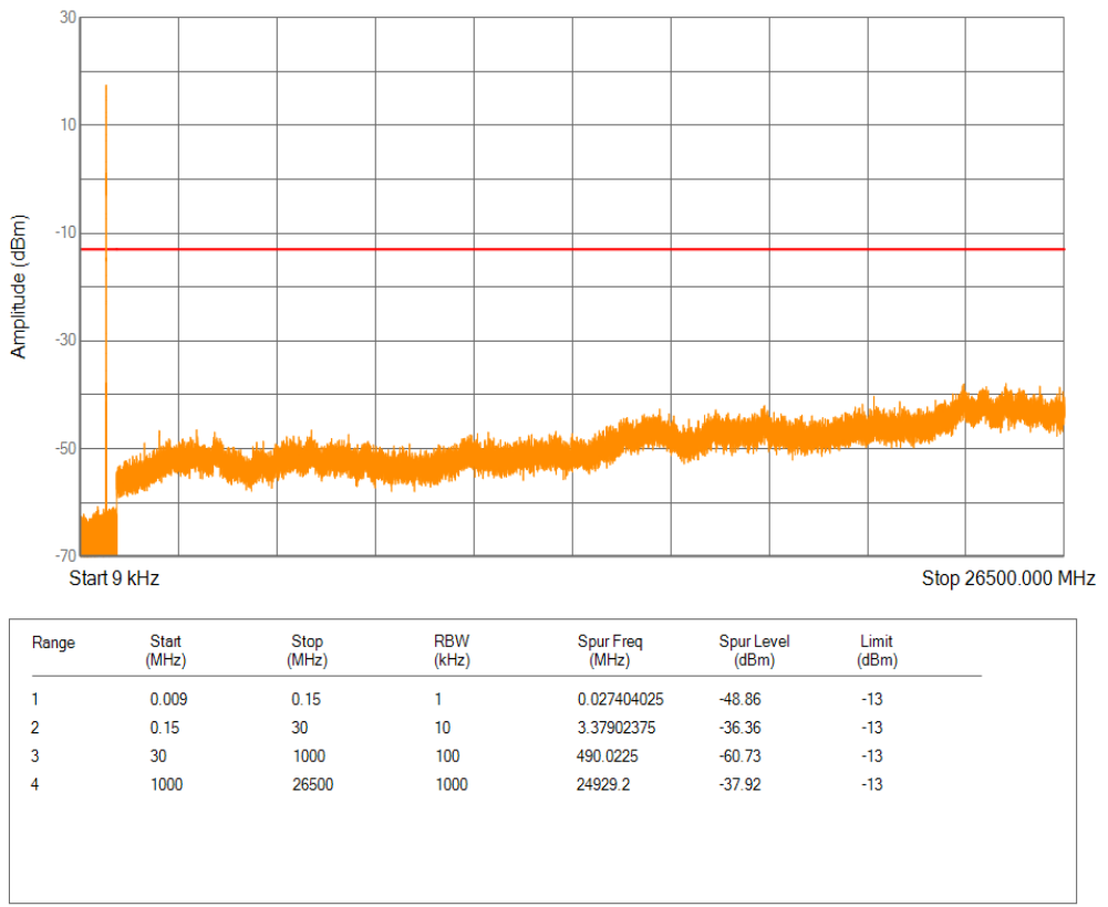
Band12 QPSK Channel=23178 nTones=1@11 Spacing=15kHz
