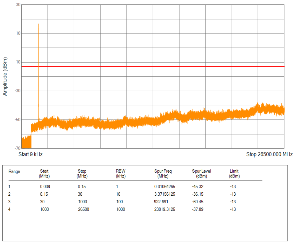
Band4 QPSK Channel=20175 nTones=1@47 Spacing=3.75kHz
