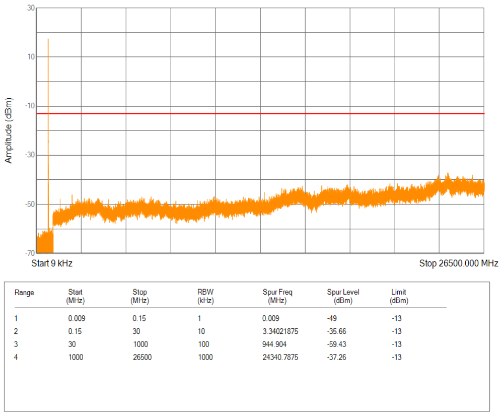
Band12 QPSK Channel=23095 nTones=1@47 Spacing=3.75kHz
