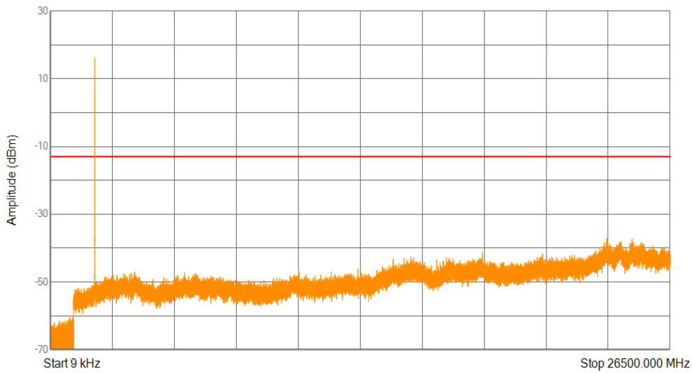
Band2 QPSK Channel=19198 nTones=1@47 Spacing=3.75kHz
