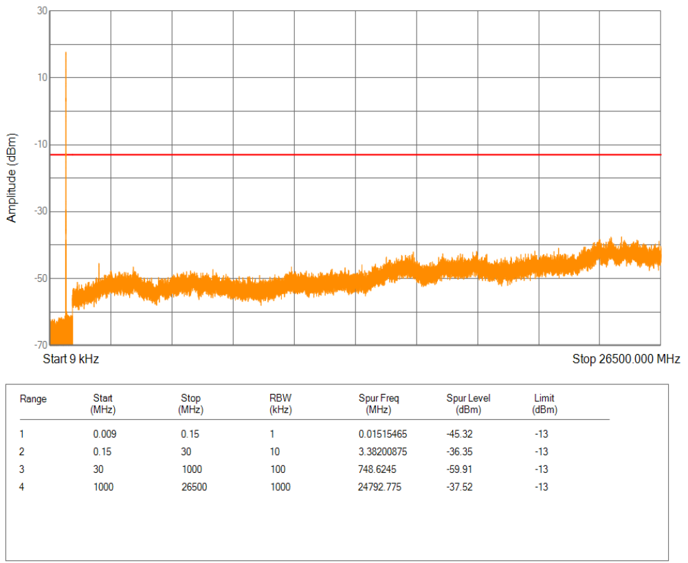
Band12 BPSK Channel=23012 nTones=1@0 Spacing=3.75kHz
