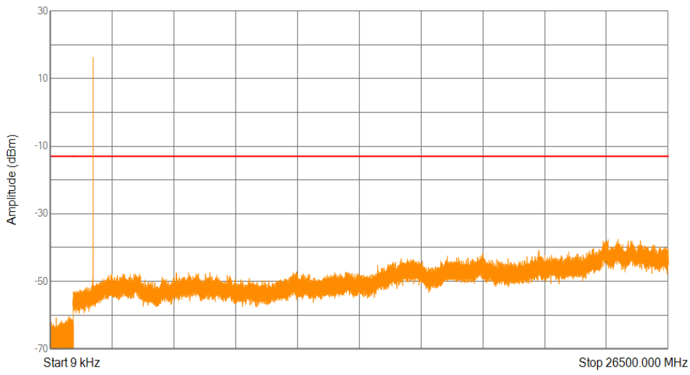
Band2 QPSK Channel=18602 nTones=1@11 Spacing=15kHz
