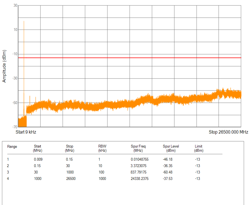
Band12 BPSK Channel=23095 nTones=1@0 Spacing=3.75kHz
