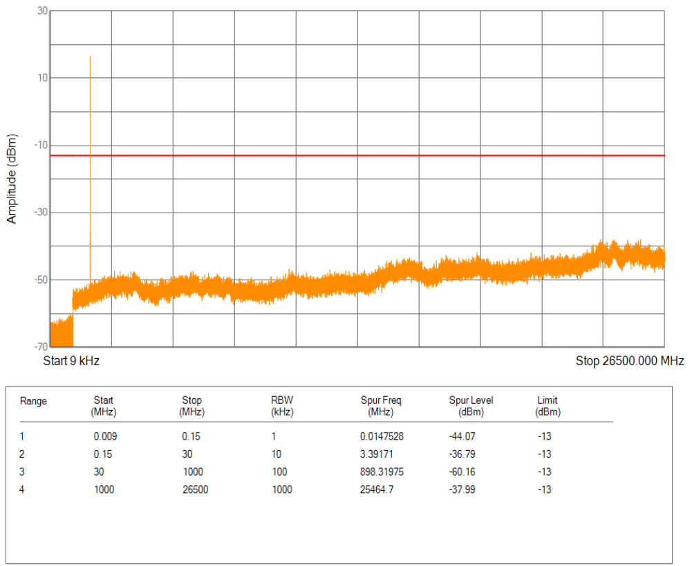
Band4 QPSK Channel=20398 nTones=1@11 Spacing=15kHz
