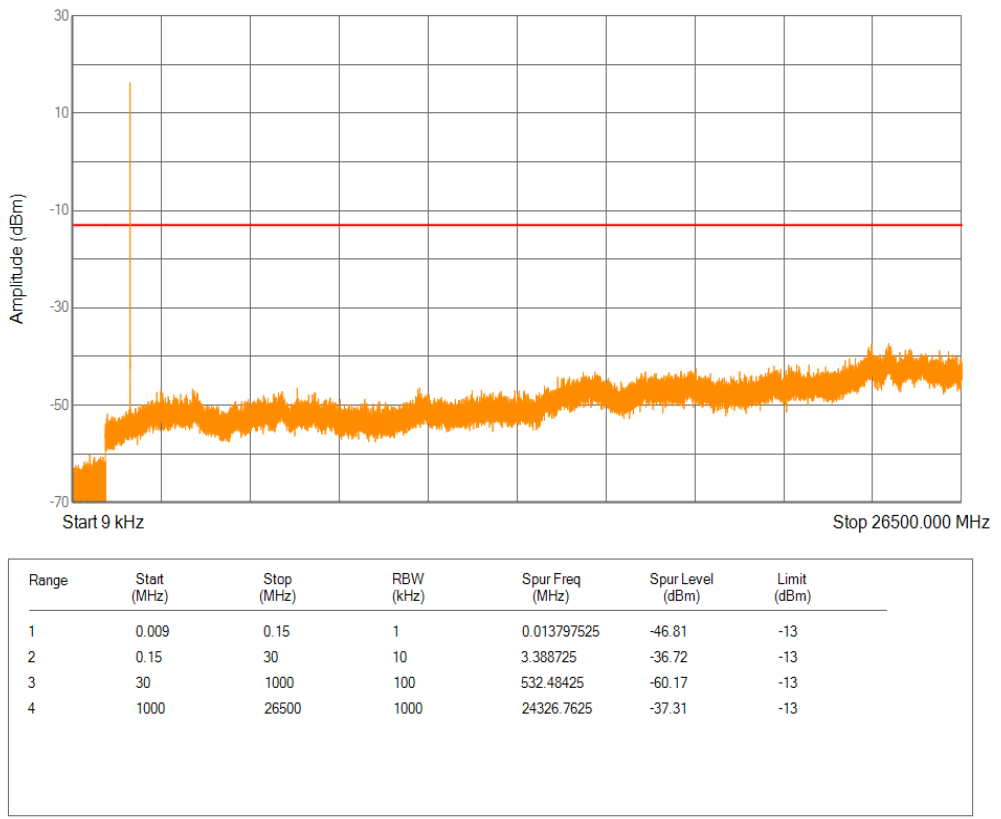
Band4 BPSK Channel=20398 nTones=1@0 Spacing=15kHz
