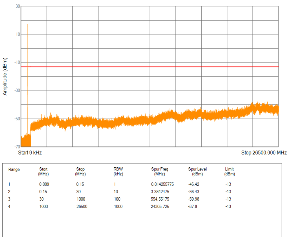
Band2 BPSK Channel=18602 nTones=1@0 Spacing=15kHz
