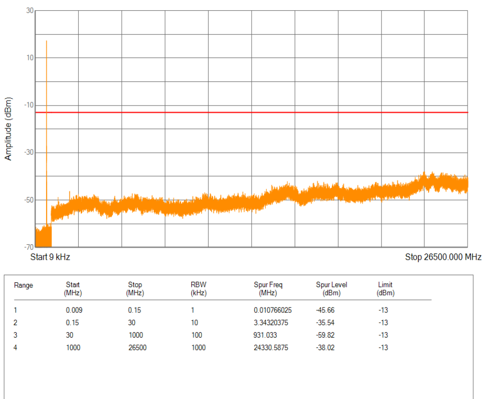
Band12 BPSK Channel=23178 nTones=1@0 Spacing=3.75kHz
