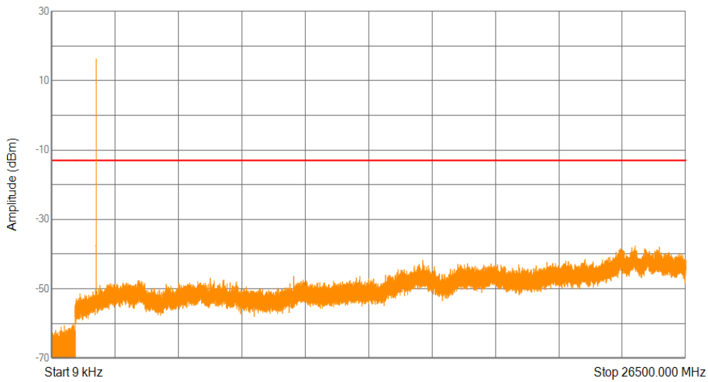
Band2 QPSK Channel=18900 nTones=1@11 Spacing=15kHz
