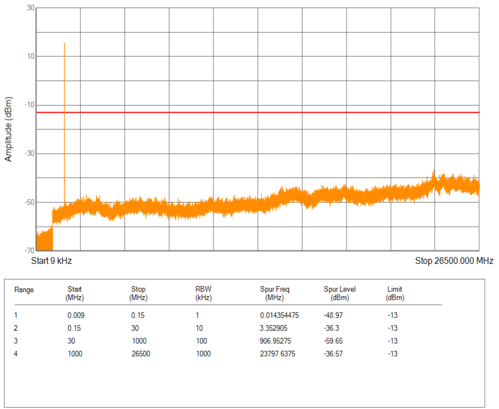
Band4 QPSK Channel=19952 nTones=1@47 Spacing=3.75kHz
