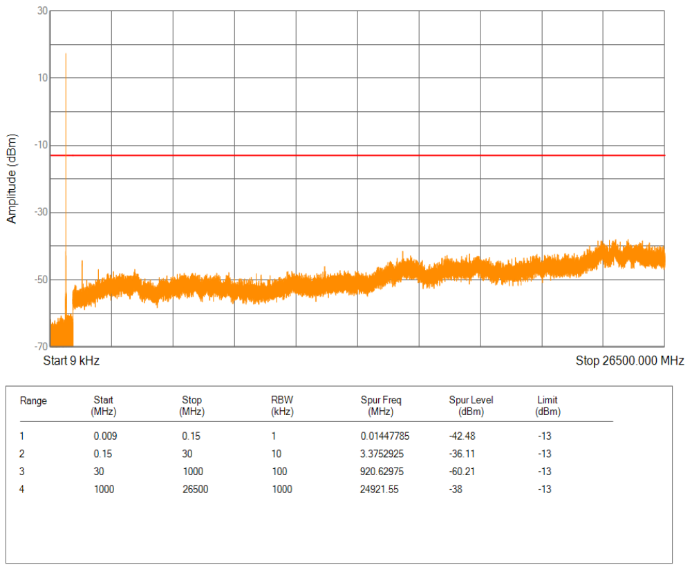
Band12 BPSK Channel=23095 nTones=1@0 Spacing=15kHz
