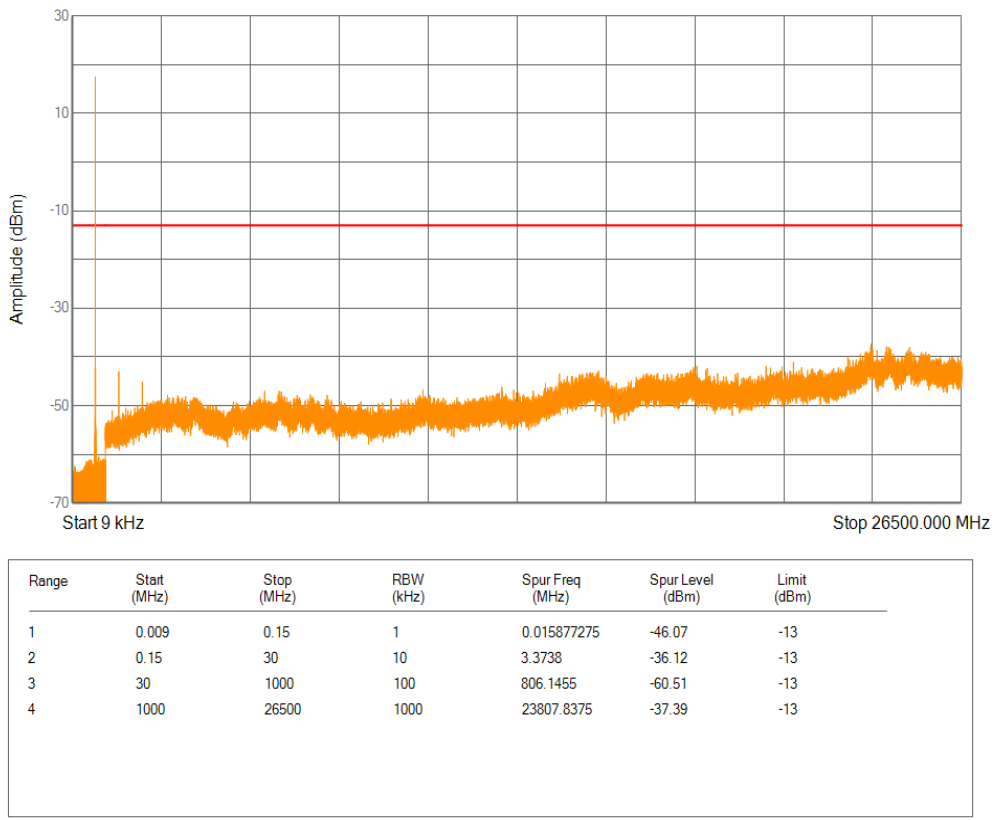
Band12 QPSK Channel=23012 nTones=1@11 Spacing=15kHz
