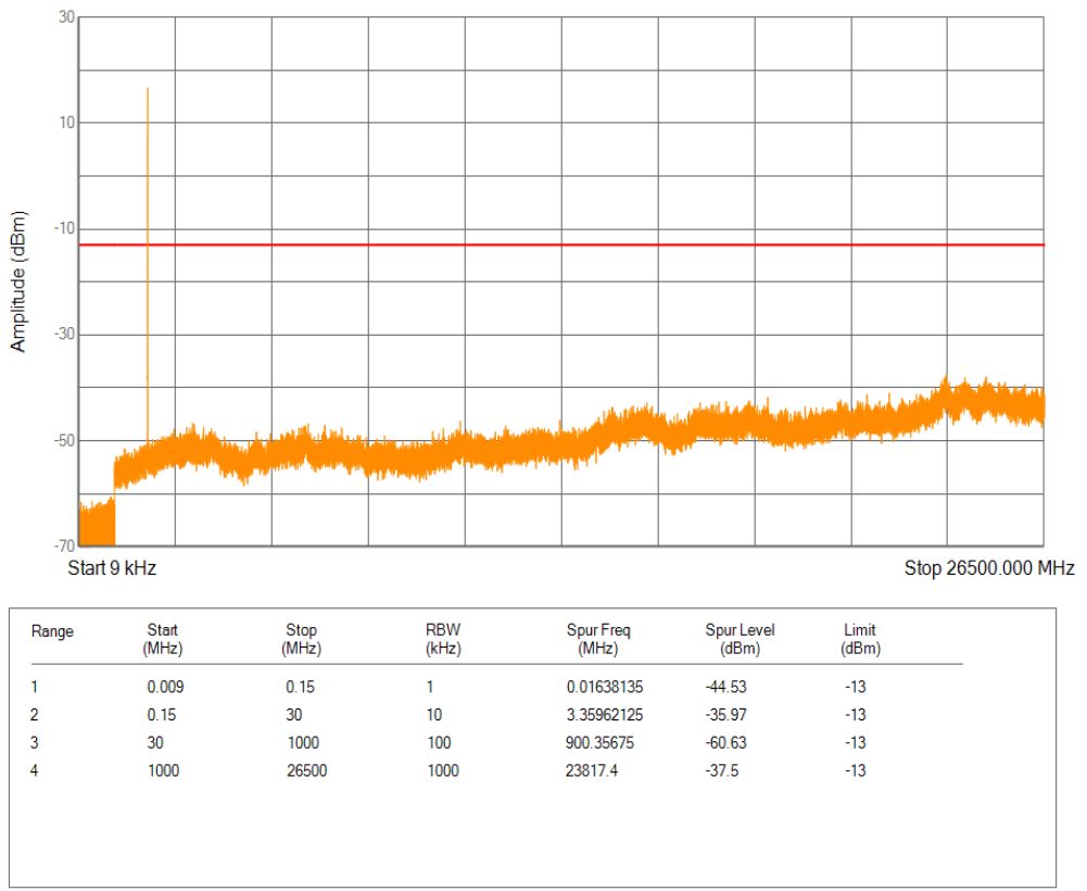
Band2 QPSK Channel=19198 nTones=1@11 Spacing=15kHz
