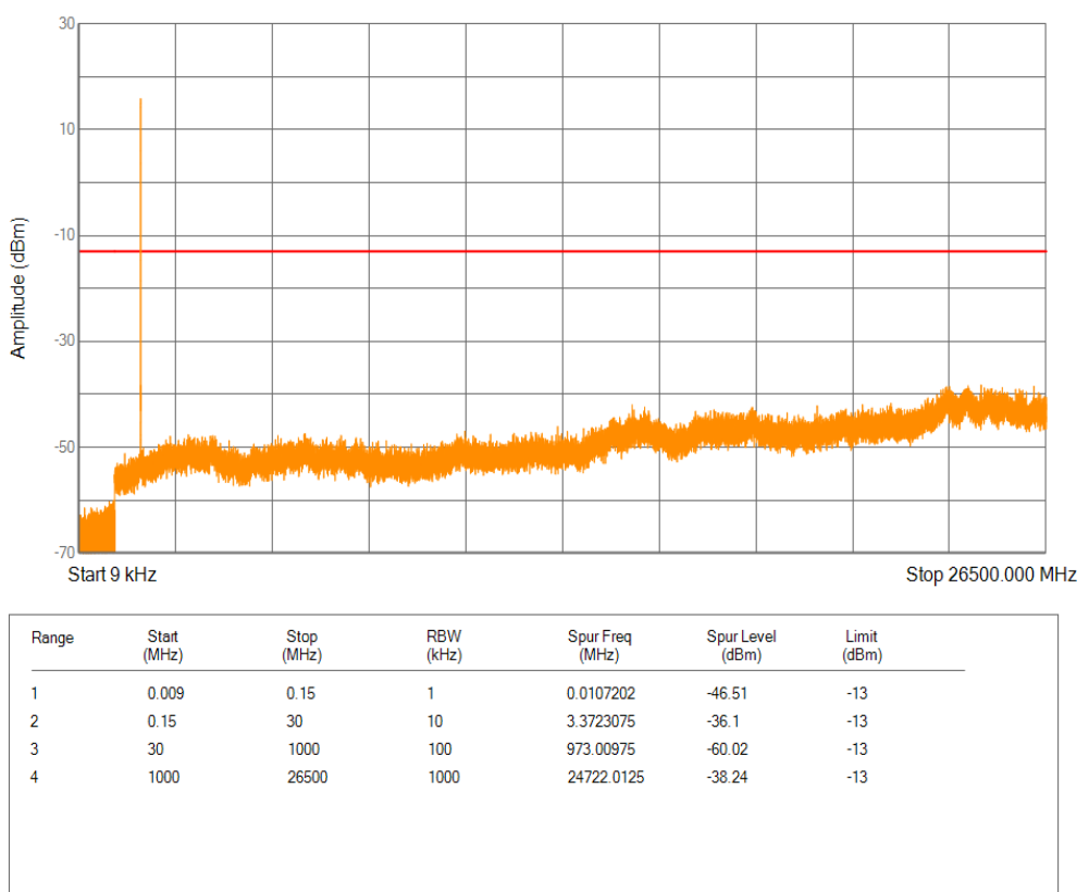
Band4 BPSK Channel=20175 nTones=1@0 Spacing=15kHz
