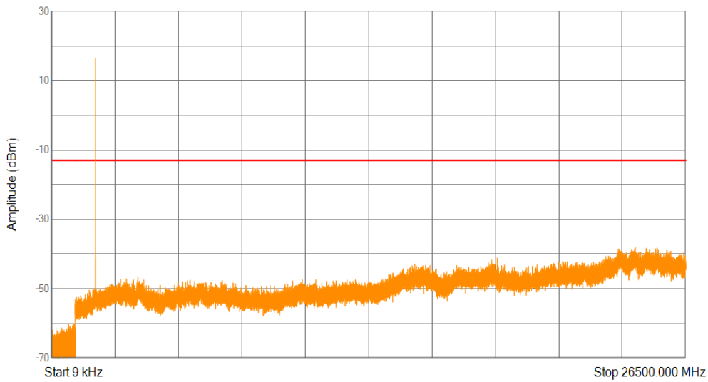
Band2 QPSK Channel=18602 nTones=1@47 Spacing=3.75kHz
