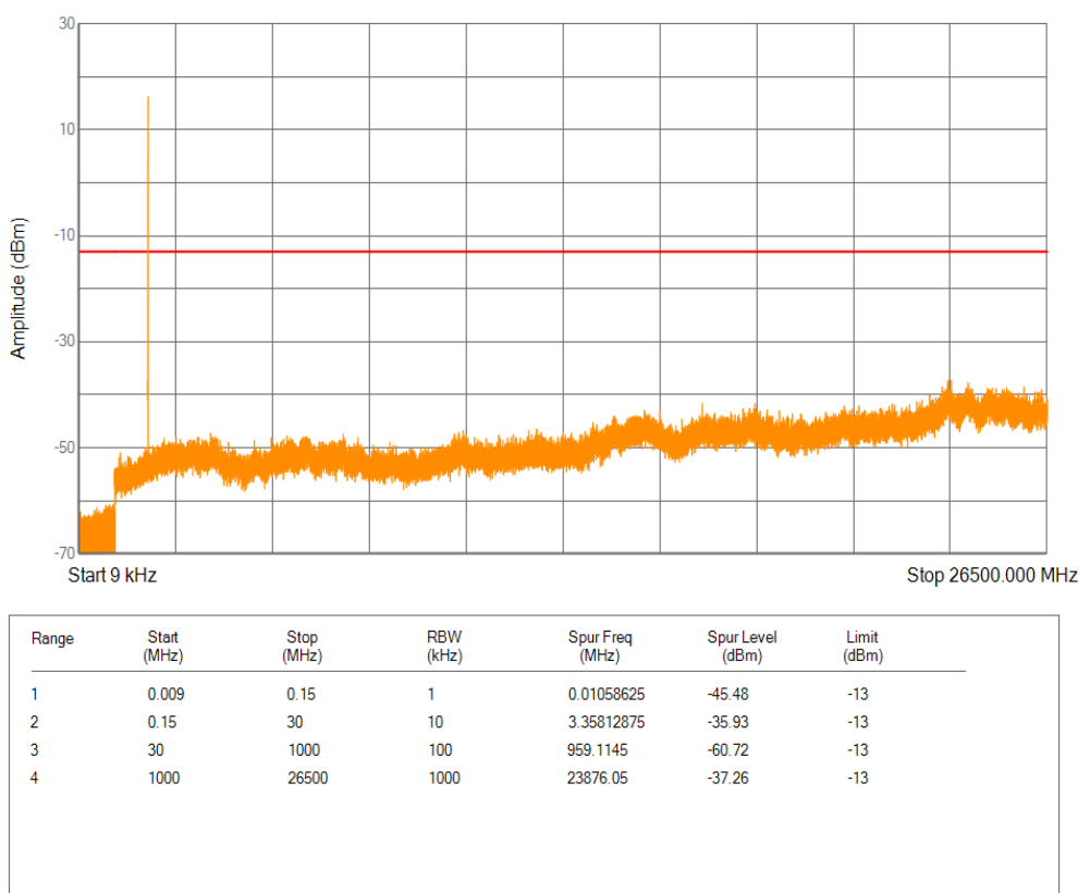
Band2 BPSK Channel=18602 nTones=1@0 Spacing=3.75kHz
