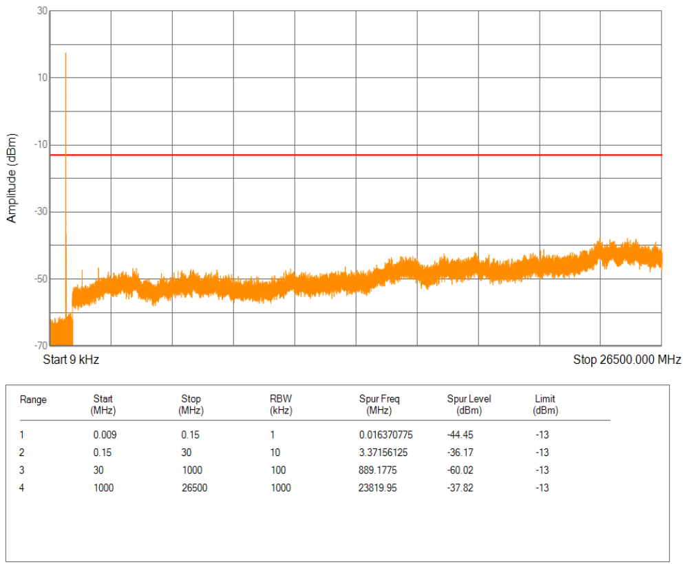
Band12 QPSK Channel=23095 nTones=1@11 Spacing=15kHz
