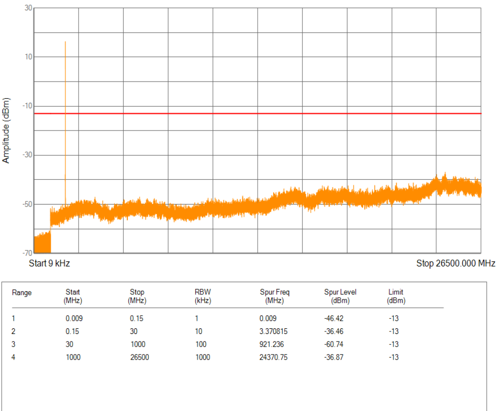
Band2 QPSK Channel=18900 nTones=1@47 Spacing=3.75kHz
