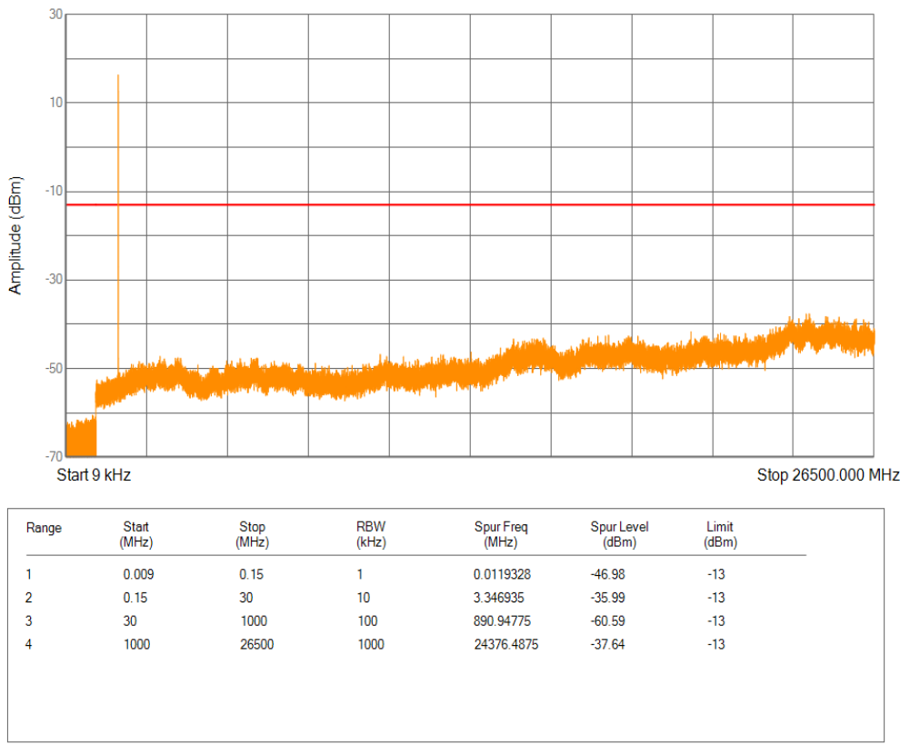
Band4 QPSK Channel=20175 nTones=1@11 Spacing=15kHz
