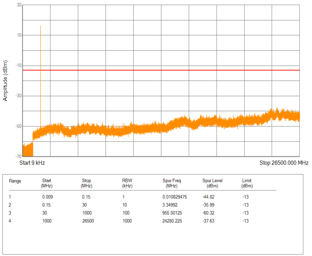
Band4 BPSK Channel=20398 nTones=1@0 Spacing=3.75kHz
