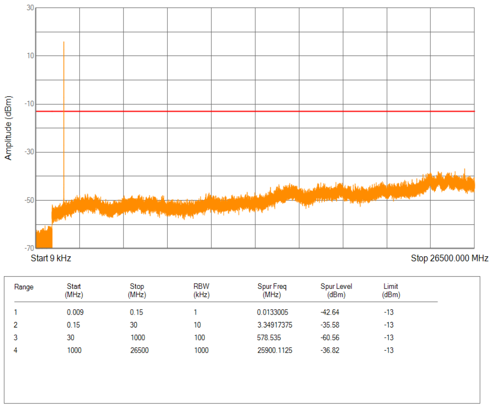
Band4 QPSK Channel=19952 nTones=1@11 Spacing=15kHz
