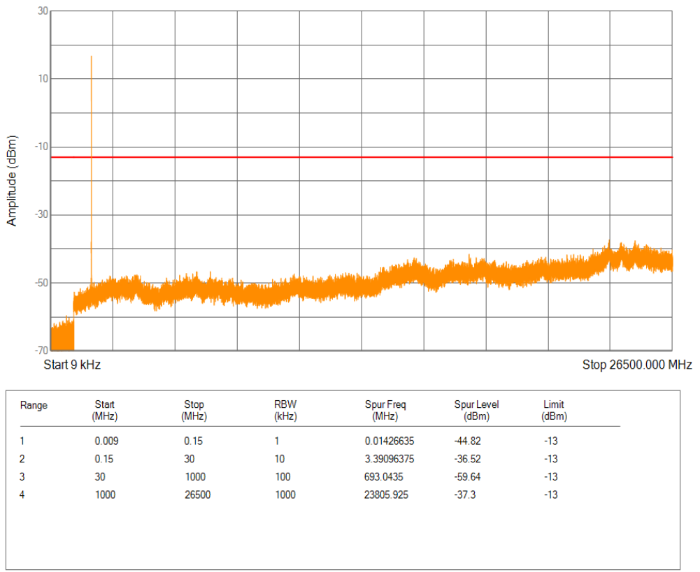
Band4 BPSK Channel=19952 nTones=1@0 Spacing=3.75kHz
