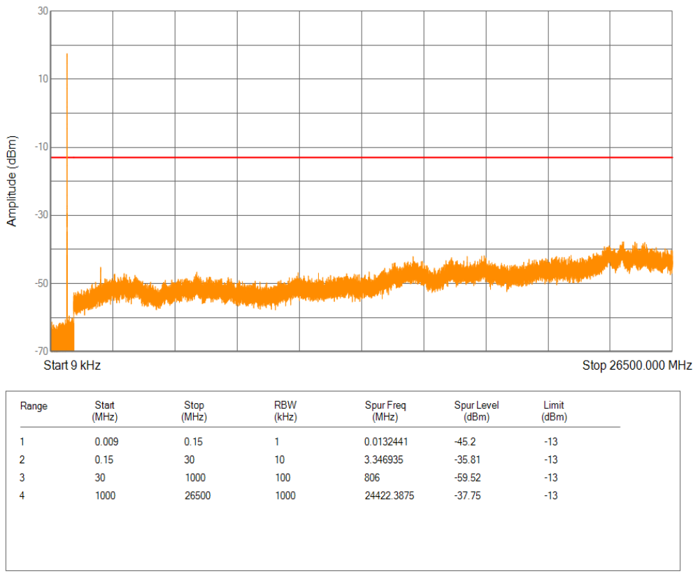
Band12 QPSK Channel=23178 nTones=1@47 Spacing=3.75kHz
