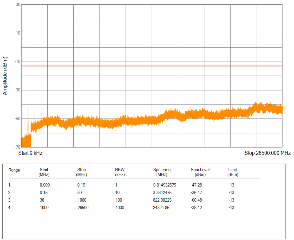
Band12 QPSK Channel=23012 nTones=1@47 Spacing=3.75kHz
