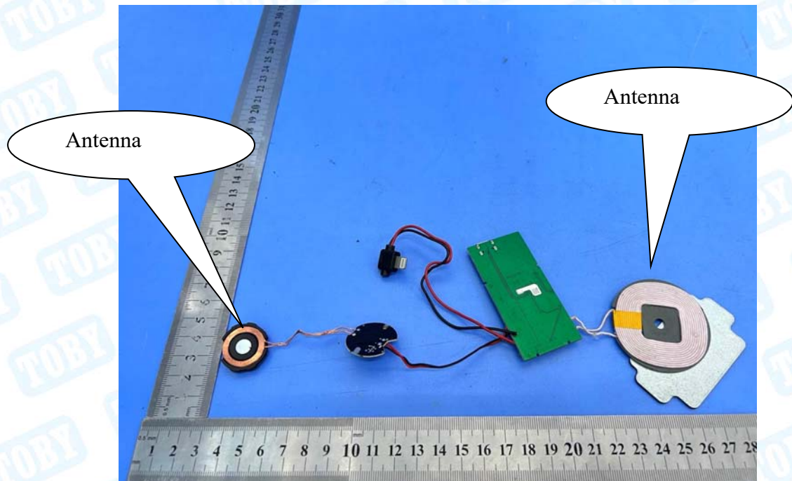
Photo 9 Appearance of PCB
