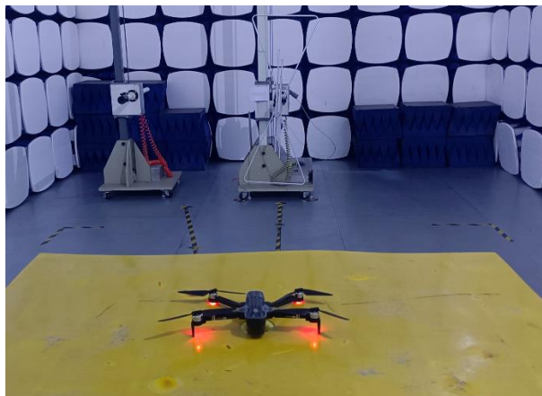
Radiated emission 30MHz~1GHz
