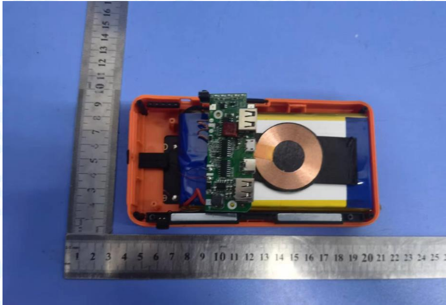
Photo 12 Internal of EUT
