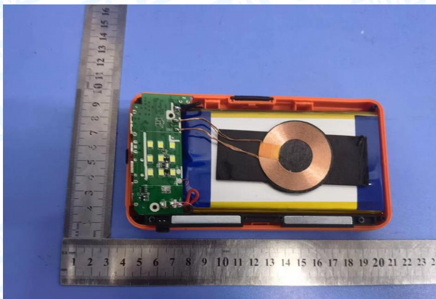
Photo 10 Internal of EUT
