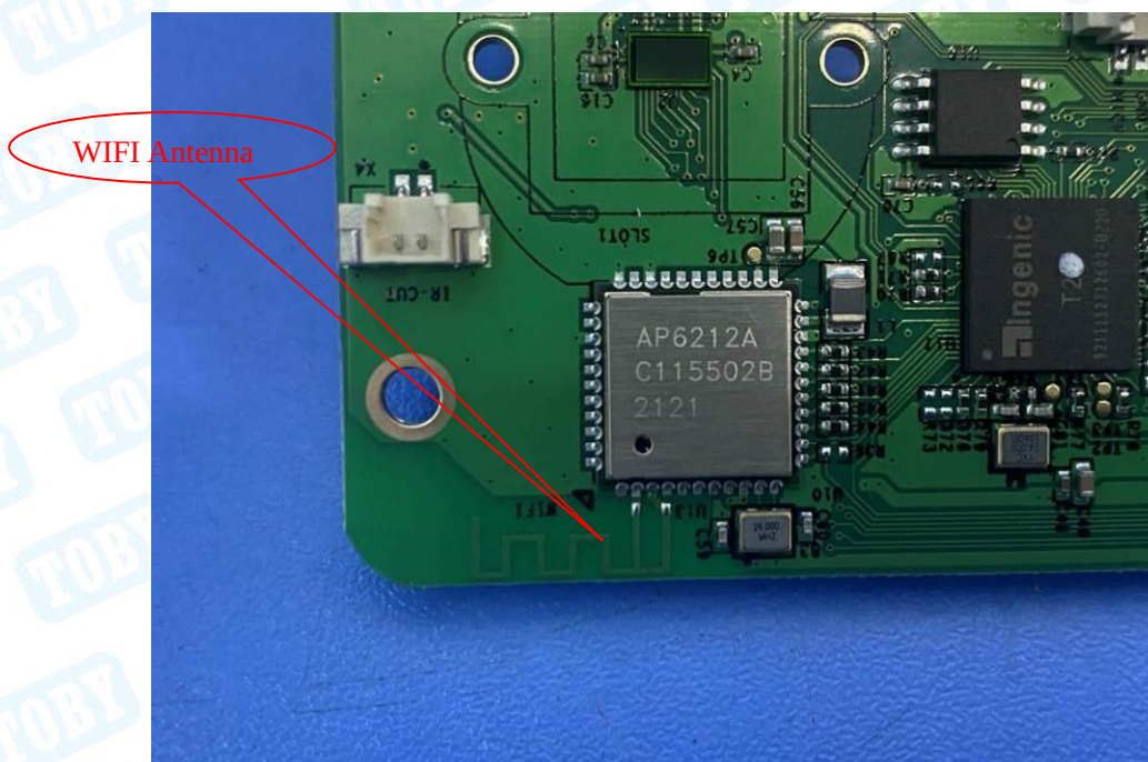
Photo 24 Appearance of PCB
