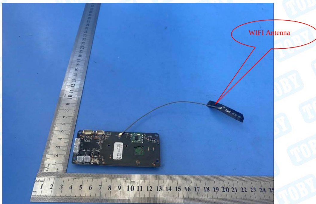
Photo 26 Appearance of PCB
