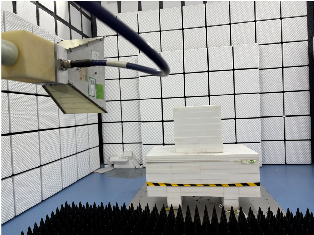
Radiated Emission - Front View (18GHz – 25GHz)
