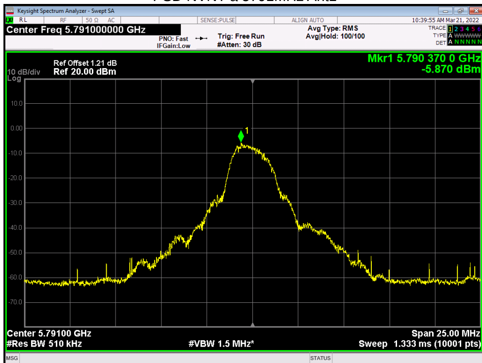
PSD NVNT a 5791MHz Ant1
