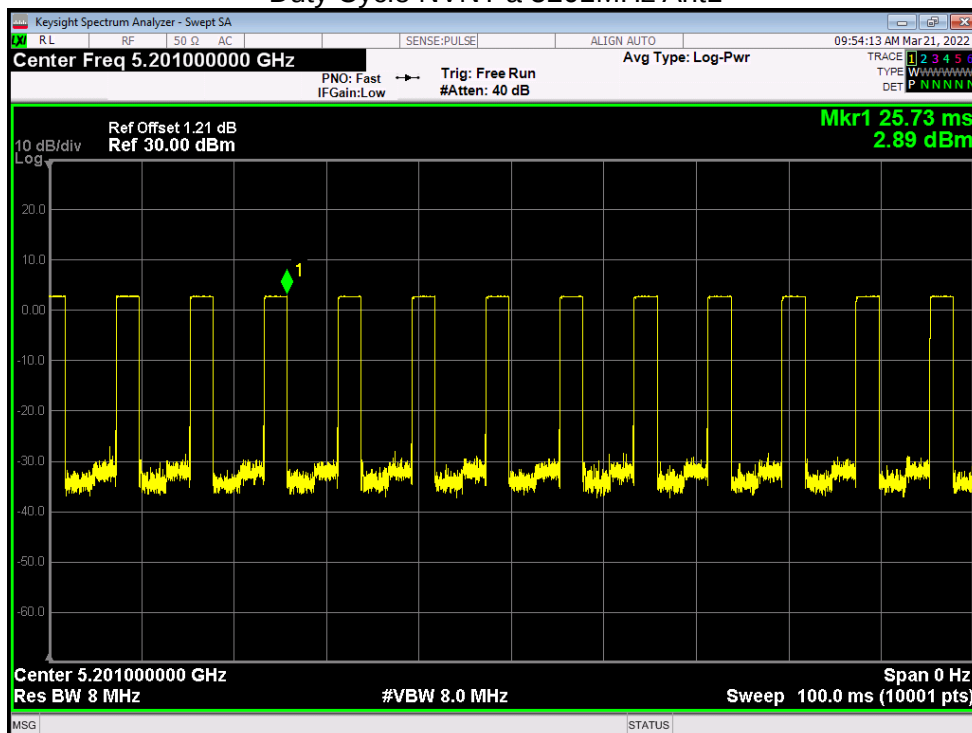
Duty Cycle NVNT a 5201MHz Ant1
