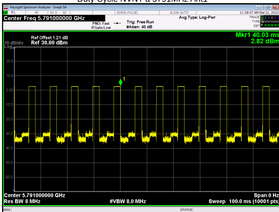
Duty Cycle NVNT a 5791MHz Ant1
