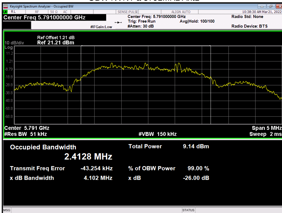
OBW NVNT a 5791MHz Ant1
