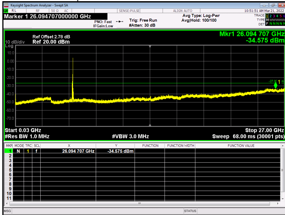
Tx. Spurious NVNT a 5791MHz Ant1 Emission
