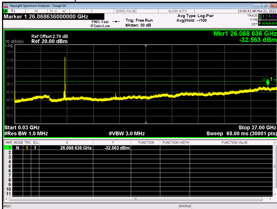
Tx. Spurious NVNT a 5201MHz Ant1 Emission
