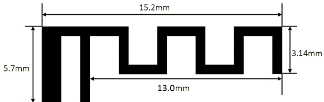
PCB Antenna
