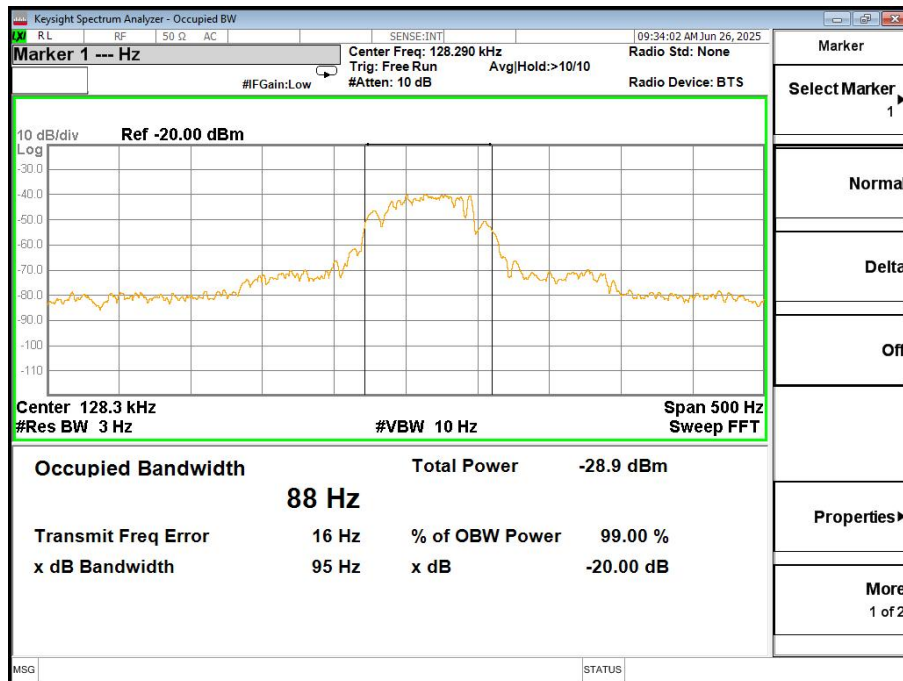
Phone coil
