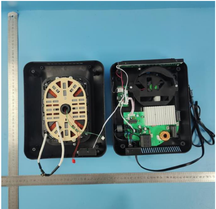
INTERNAL PHOTO OF SAMPLE
