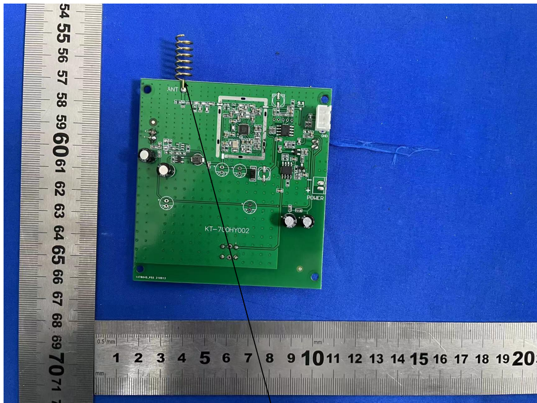
Integral Antenna
