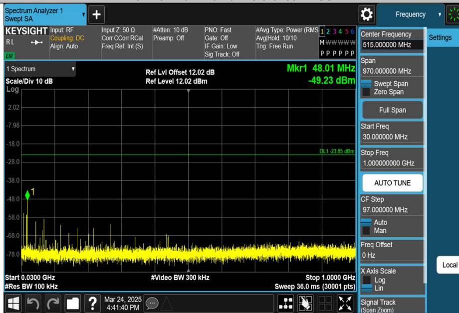
3DH5-Ant1-2402-30~1000-PASS
