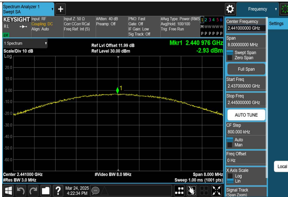
2DH5-Ant1-2441-PASS
