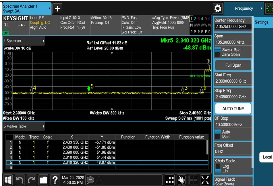
3DH5-Ant1-Hop_2402-PASS
