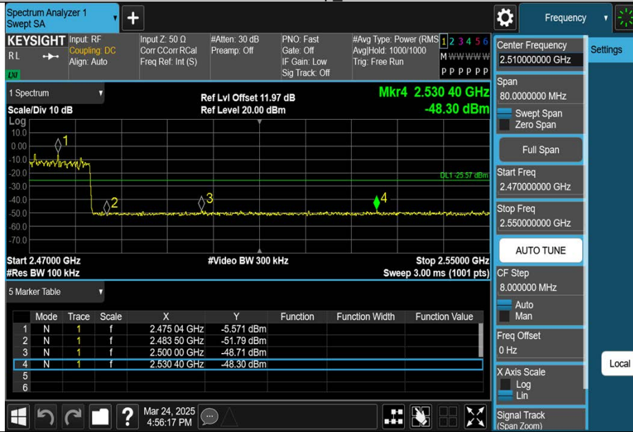
2DH5-Ant1-Hop_2480-PASS
