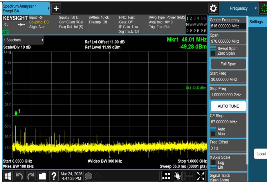
3DH5-Ant1-2441-30~1000-PASS
