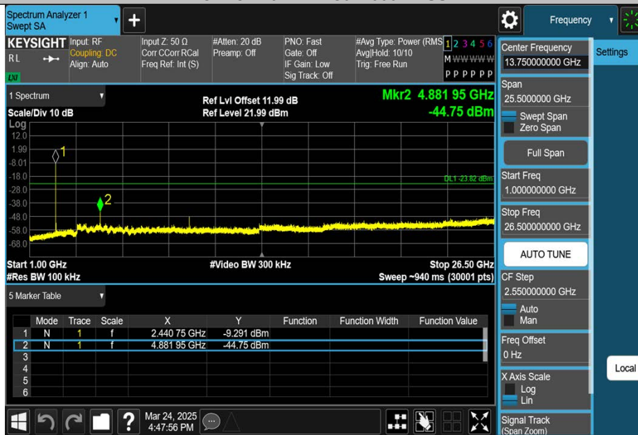
3DH5-Ant1-2441-1000~26500-PASS
