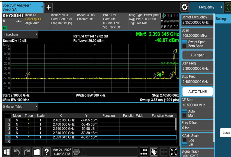
3DH5-Ant1-2402-PASS
