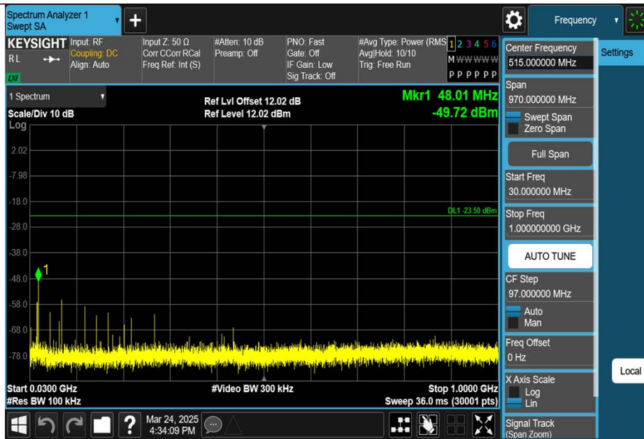
2DH5-Ant1-2402-30~1000-PASS
