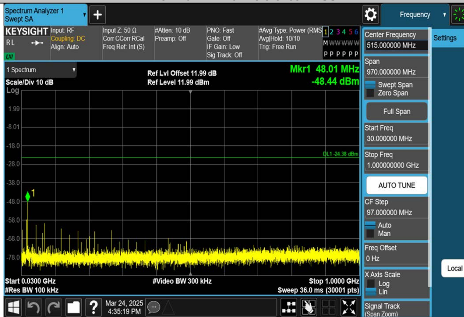
2DH5-Ant1-2441-30~1000-PASS
