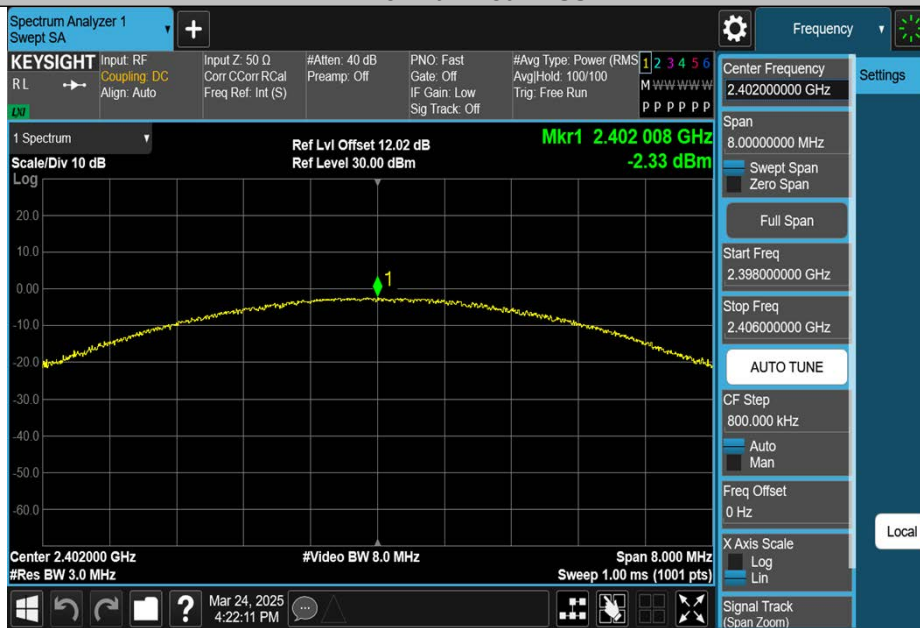
2DH5-Ant1-2402-PASS
