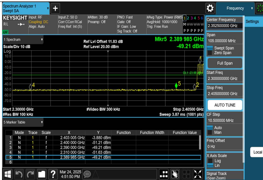
DH5-Ant1-Hop_2402-PASS
