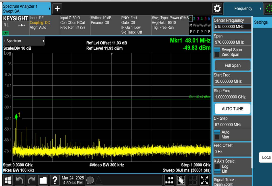
3DH5-Ant1-2480-30~1000-PASS
