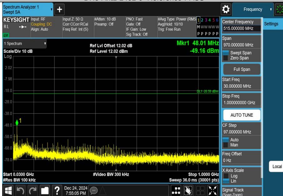
DH5-Ant1-2402-30~1000-PASS
