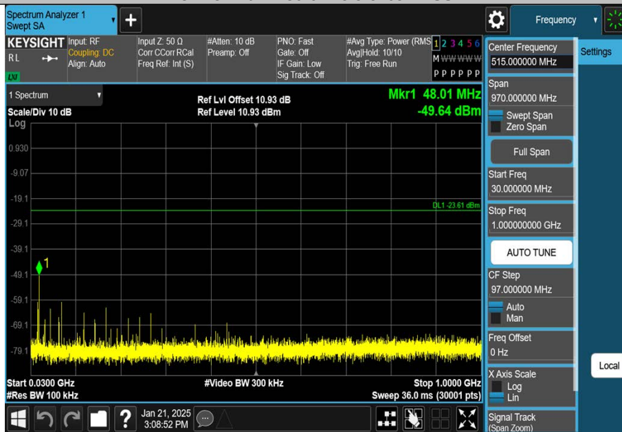
3DH5-Ant1-2480-30~1000-PASS
