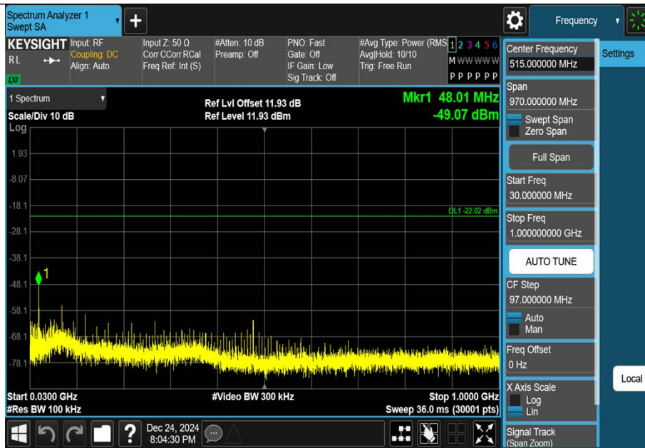
2DH5-Ant1-2480-30~1000-PASS
