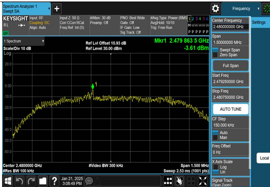
3DH5-Ant1-2480-0~Reference-PASS
