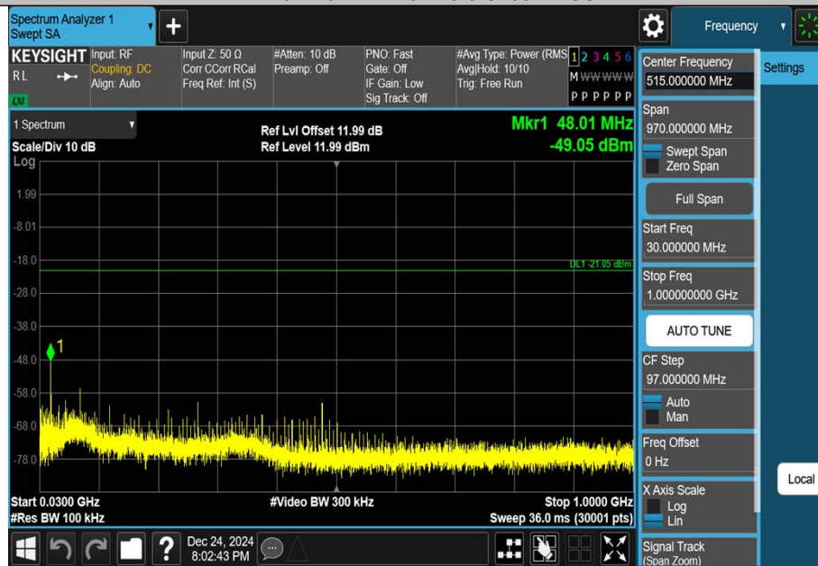
2DH5-Ant1-2441-30~1000-PASS
