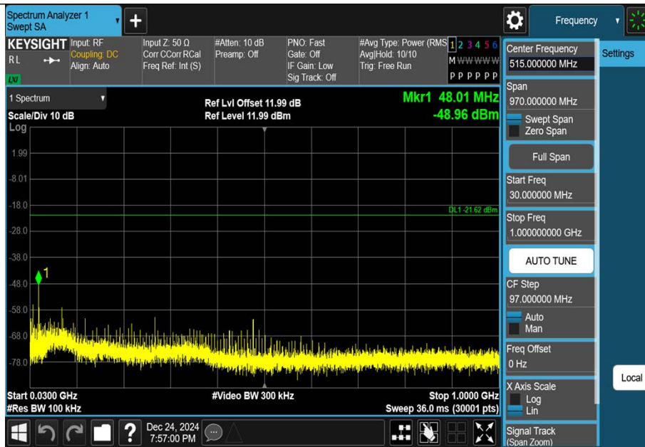
DH5-Ant1-2441-30~1000-PASS
