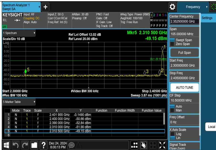
2DH5-Ant1-2402-PASS
