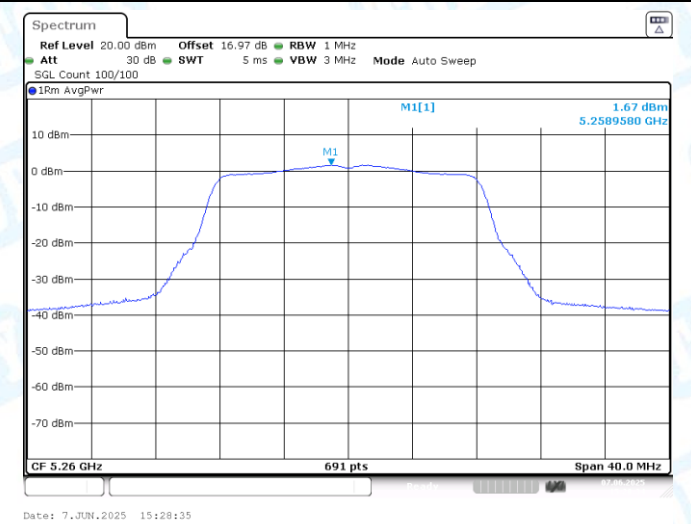
11A-Ant1-5260-PASS
