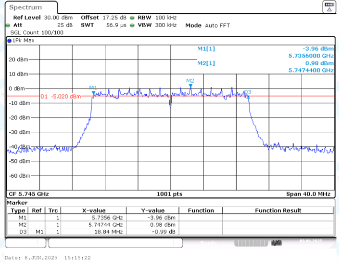
11AX20SISO-Ant1-5745-PASS
