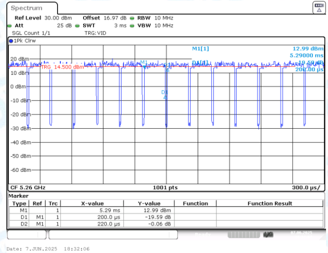
NTNV-11AC20SISO-Ant1-5260
