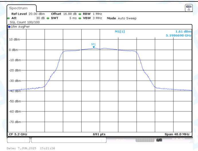
11A-Ant1-5200-PASS
