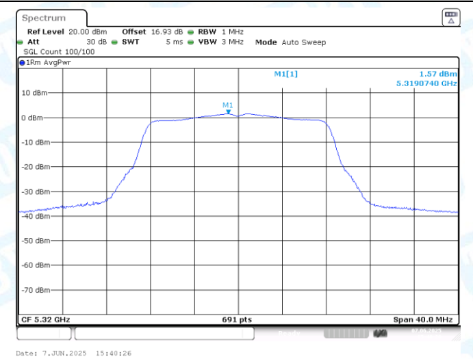
11A-Ant1-5320-PASS
