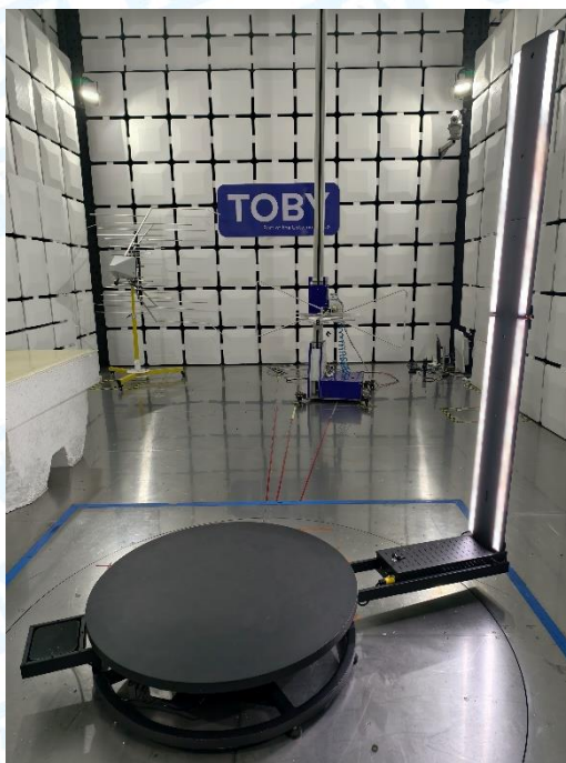
Radiated Emission Test Setup-Below 1G
