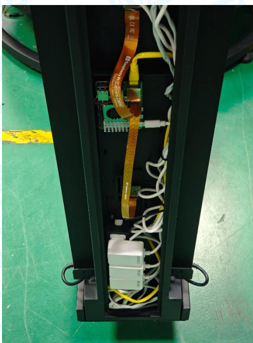
Photo 40 Internal of EUT
