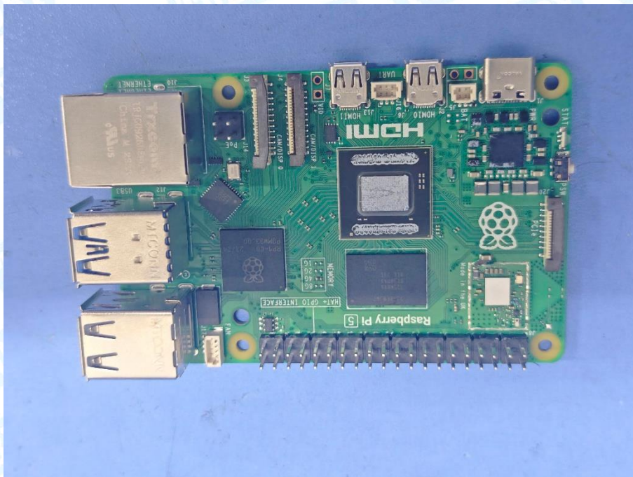
Photo 52 Appearance of PCB
