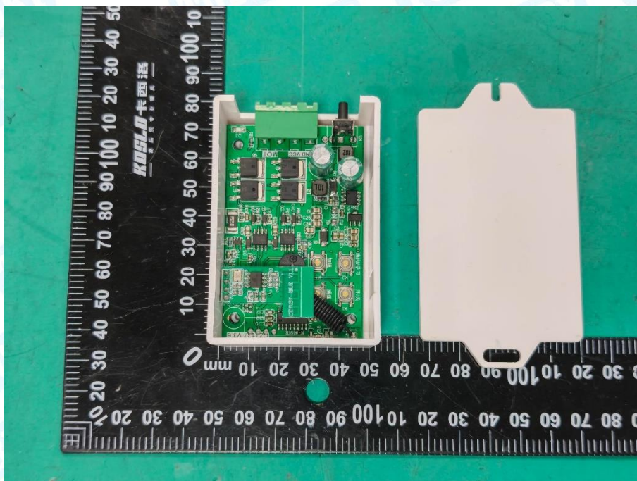
Photo 58 Internal of EUT
