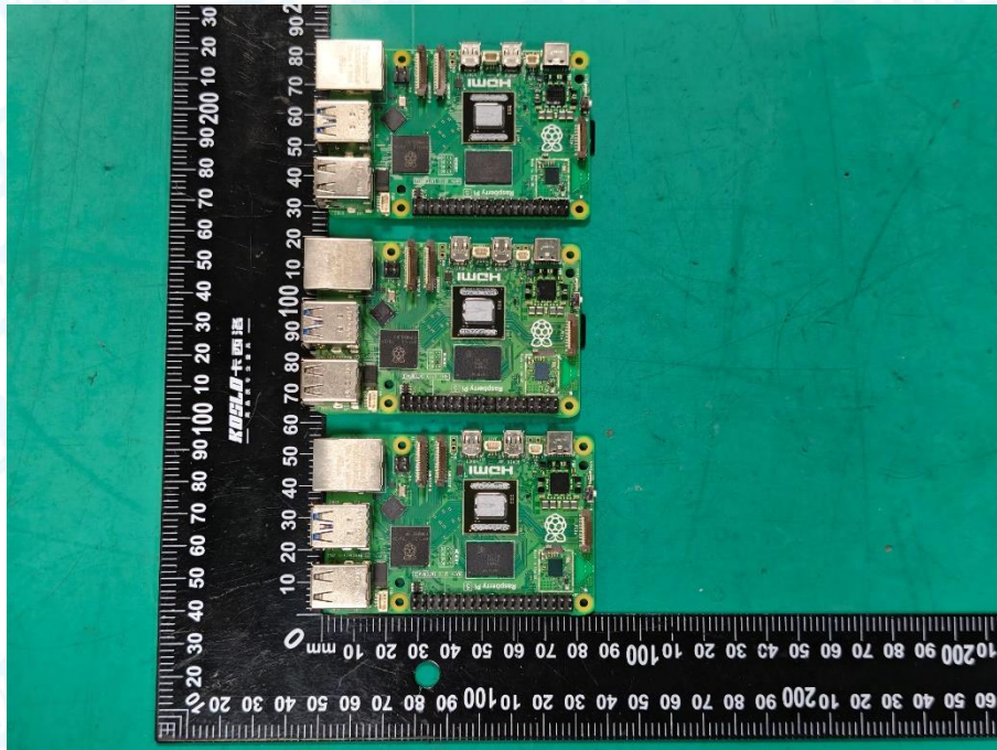
Photo 56 Appearance of PCB
