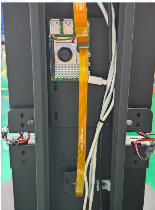
Photo 42 Internal of EUT
