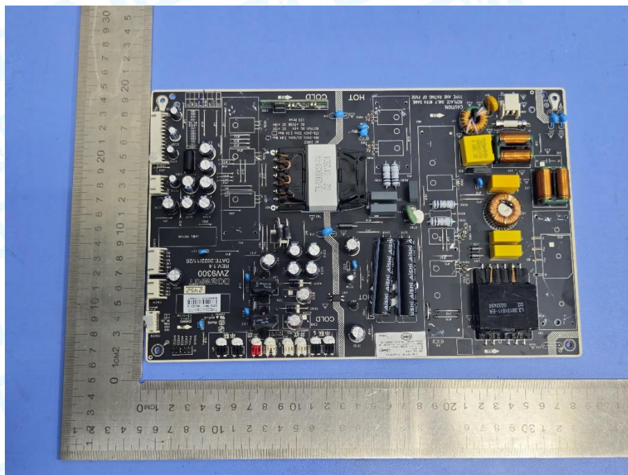
Photo 35 Appearance of PCB
