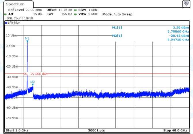
11AX80MIMO-Ant2-5775-1000~40000-PASS
