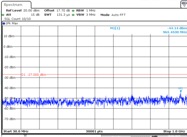
11AX80MIMO-Ant1-5610-30~1000-PASS
