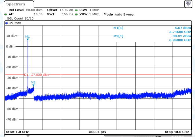
11AX40MIMO-Ant2-5755-1000~40000-PASS
