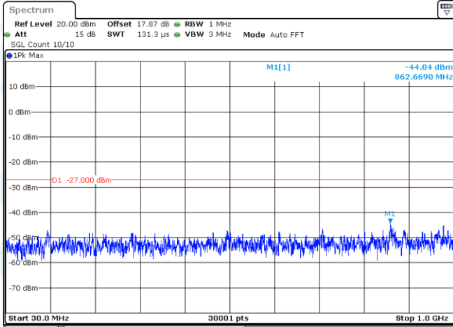
11AX40MIMO-Ant1-5670-30~1000-PASS
