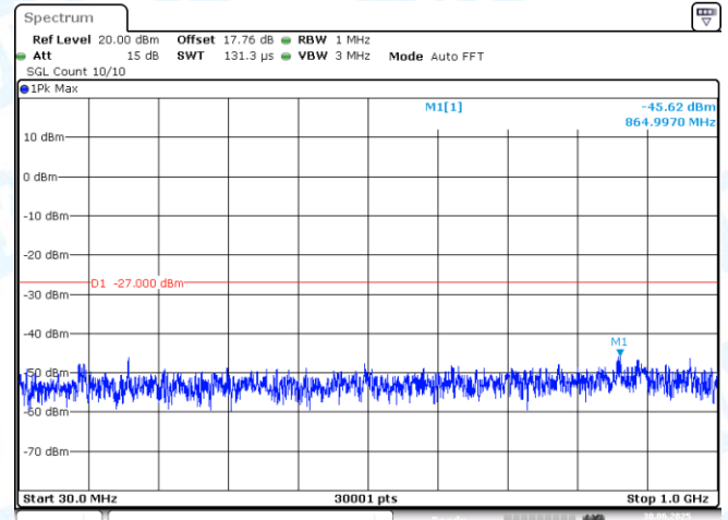
11AX80MIMO-Ant2-5610-30~1000-PASS
