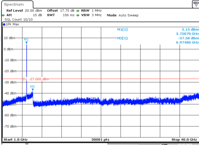
11AX40MIMO-Ant1-5755-1000~40000-PASS
