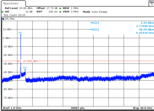
11AX80MIMO-Ant1-5775-1000~40000-PASS
