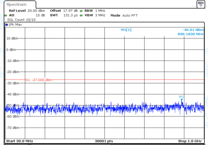
11AX40MIMO-Ant2-5670-30~1000-PASS
