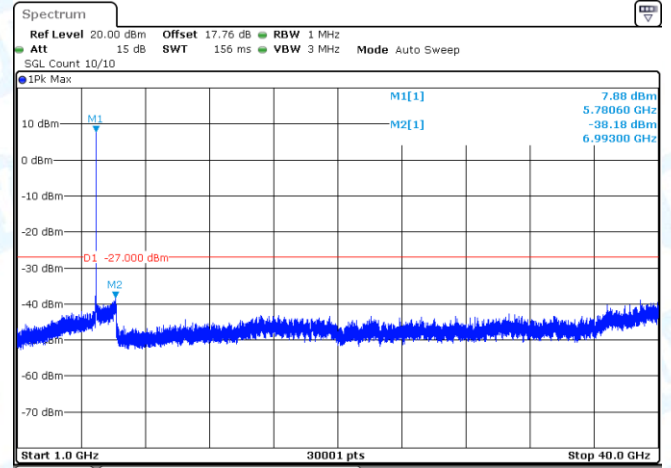
11AX20MIMO-Ant2-5785-1000~40000-PASS
