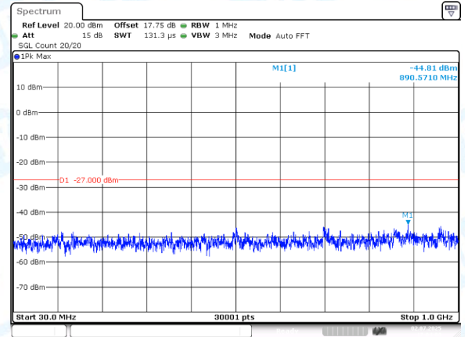
11AX20MIMO-Ant2-5745-30~1000-PASS
