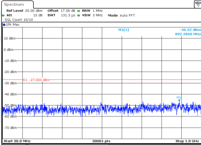
11AX20MIMO-Ant1-5500-30~1000-PASS
