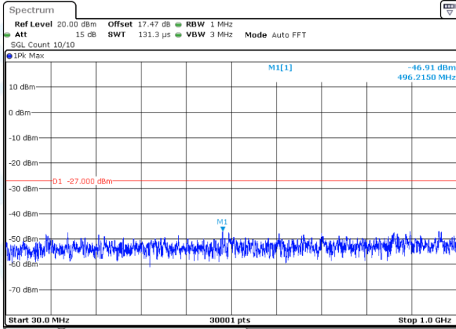
11AX20MIMO-Ant1-5260-30~1000-PASS
