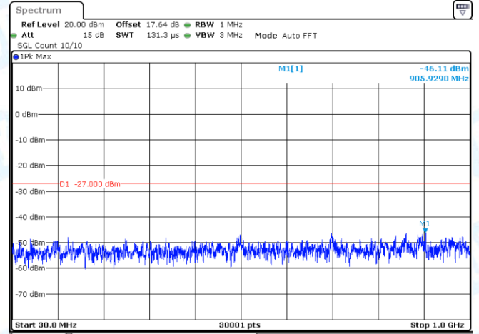
11AX20MIMO-Ant2-5500-30~1000-PASS
