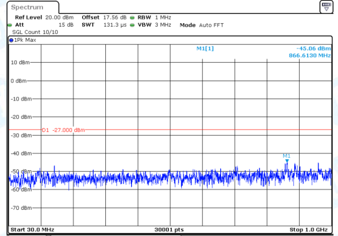
11AX20MIMO-Ant2-5260-30~1000-PASS
