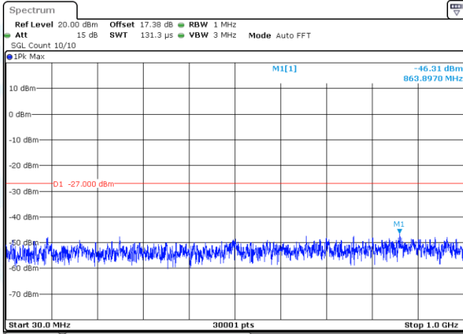
11AX40MIMO-Ant1-5190-30~1000-PASS
