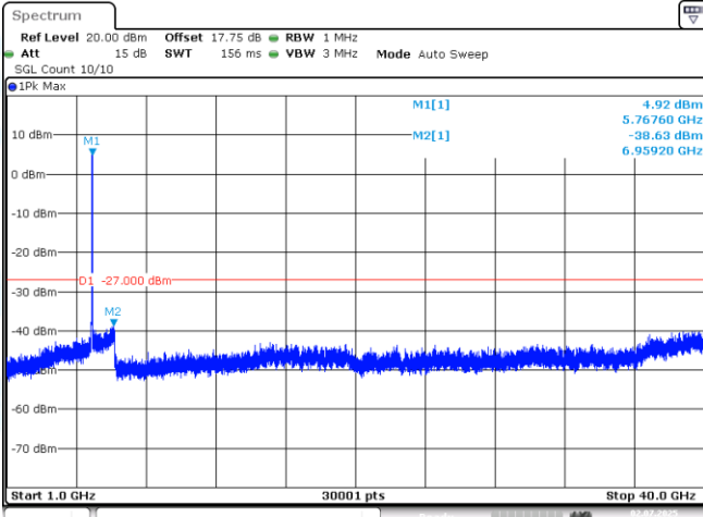
11N40MIMO-Ant1-5755-1000~40000-PASS
