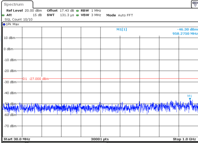
11AX40MIMO-Ant1-5310-30~1000-PASS
