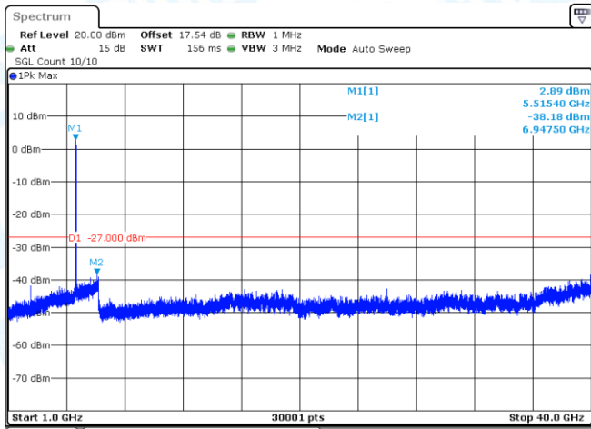
11AX40MIMO-Ant1-5510-1000~40000-PASS
