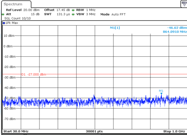
11AX20MIMO-Ant1-5180-30~1000-PASS
