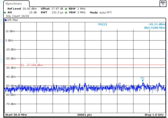
11N40MIMO-Ant2-5670-30~1000-PASS
