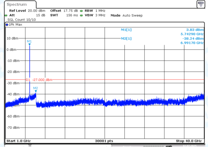
11N40MIMO-Ant2-5755-1000~40000-PASS
