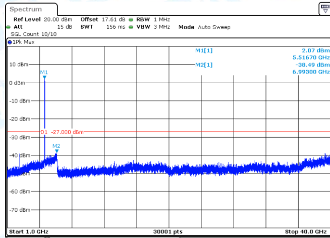
11AX40MIMO-Ant2-5510-1000~40000-PASS
