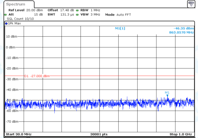
11AX40MIMO-Ant2-5190-30~1000-PASS
