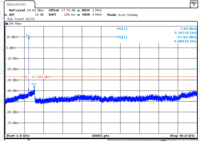
11N20MIMO-Ant2-5785-1000~40000-PASS
