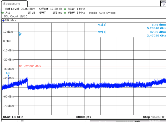
11AX20MIMO-Ant1-5200-1000~40000-PASS
