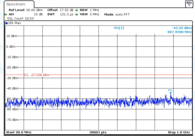
11N40MIMO-Ant2-5310-30~1000-PASS
