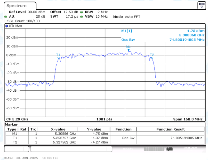
11AX80MIMO-Ant2-5290
