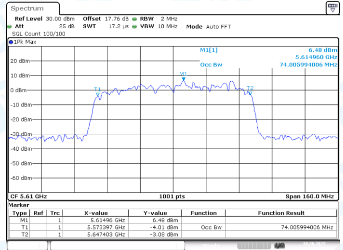
11AX80MIMO-Ant2-5610
