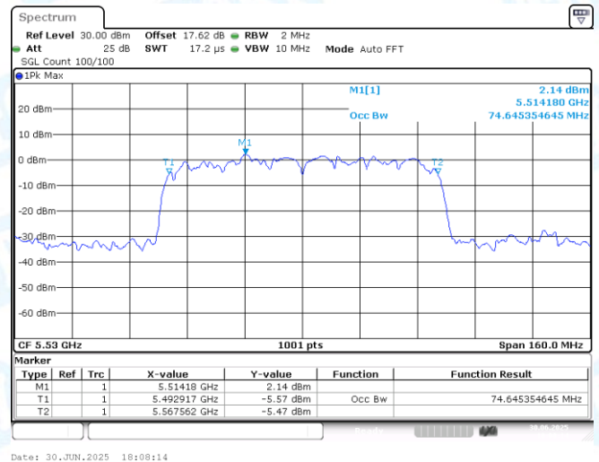
11AX80MIMO-Ant2-5530
