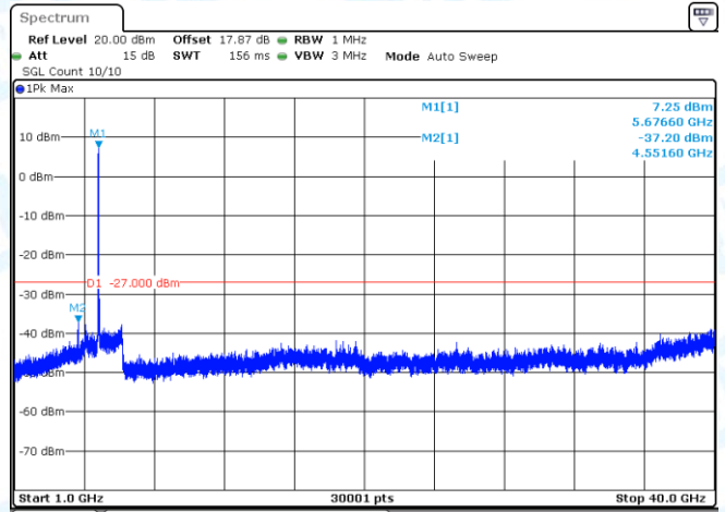
11AX40SISO-Ant1-5670-1000~40000-PASS
