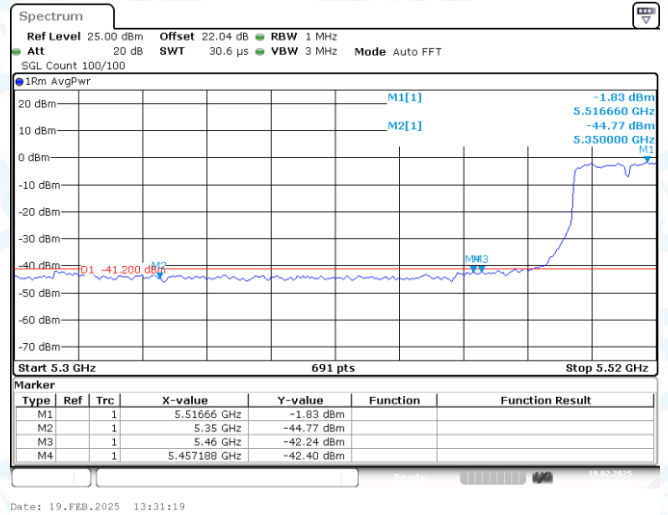
11N40SISO-Ant1-5510-PASS
