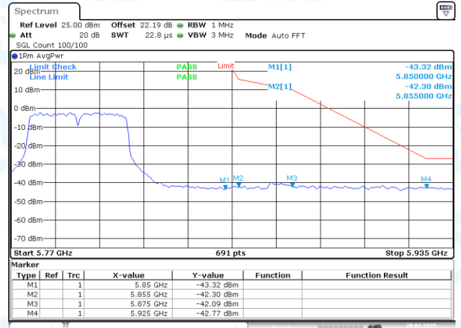
11AC40SISO-Ant1-5795-PASS
