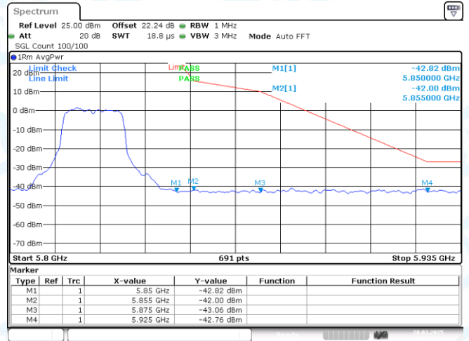
11N20SISO-Ant1-5825-PASS
