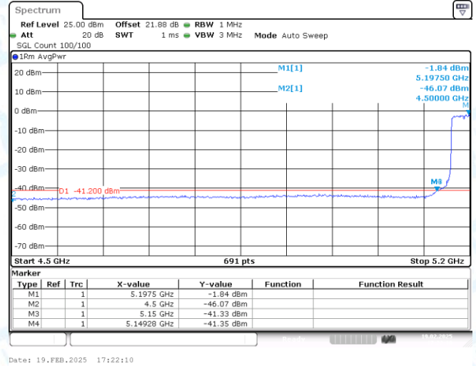
11AX40SISO-Ant1-5190-PASS
