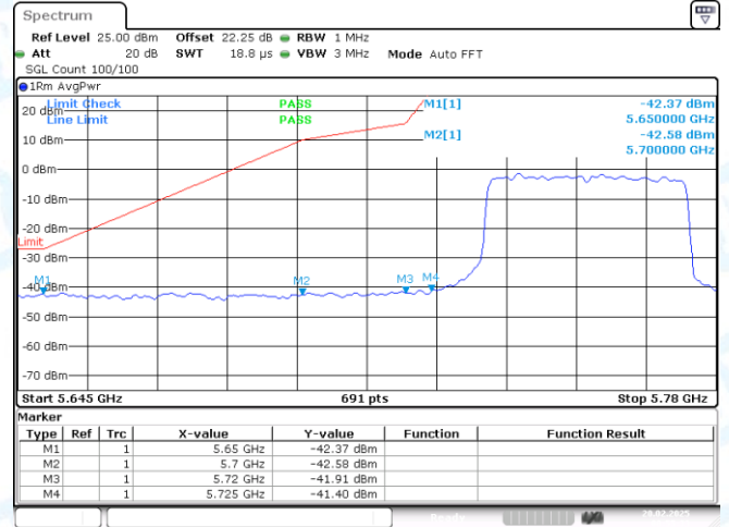
11AX40SISO-Ant1-5755-PASS
