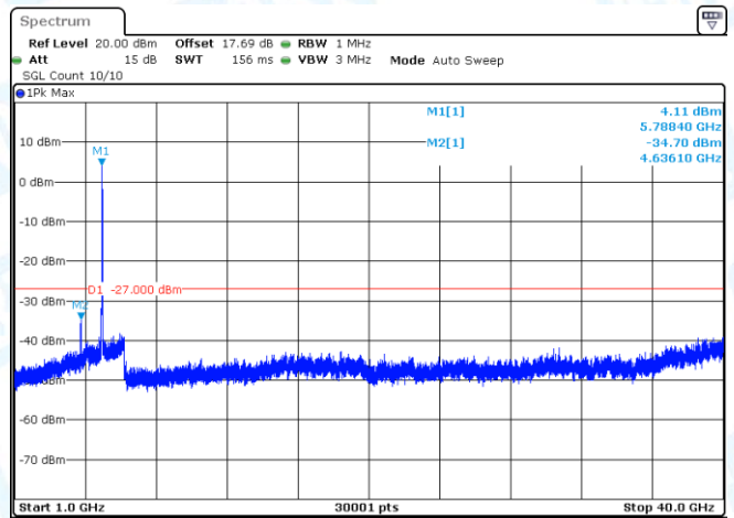
11AX40SISO-Ant1-5755-1000~40000-PASS
