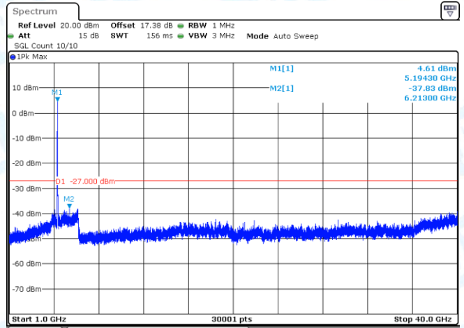
11AC40SISO-Ant1-5190-1000~40000-PASS
