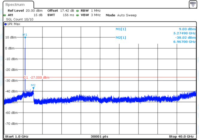
11AX20SISO-Ant1-5260-1000~40000-PASS
