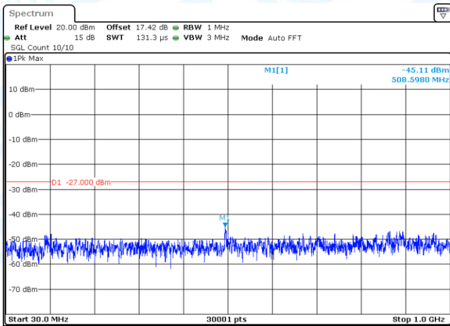
11AC40SISO-Ant1-5230-30~1000-PASS
