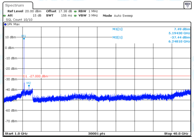
11AX20SISO-Ant1-5180-1000~40000-PASS
