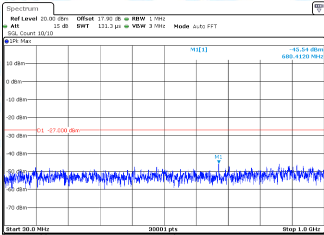
11N20SISO-Ant1-5580-30~1000-PASS
