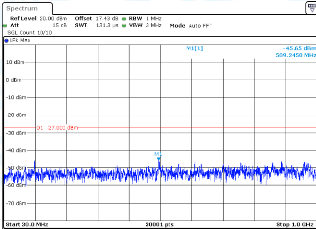
11N20SISO-Ant1-5280-30~1000-PASS
