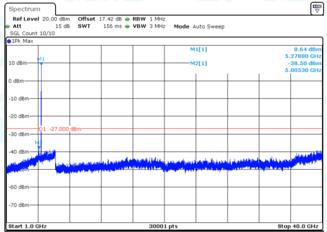
11AC20SISO-Ant1-5260-1000~40000-PASS
