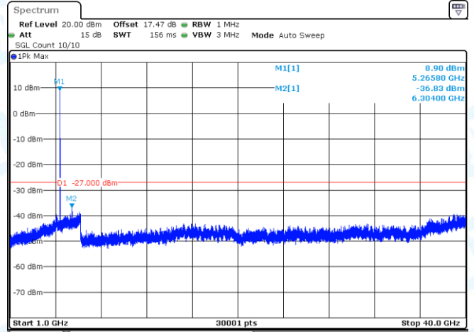
11N20SISO-Ant1-5260-1000~40000-PASS
