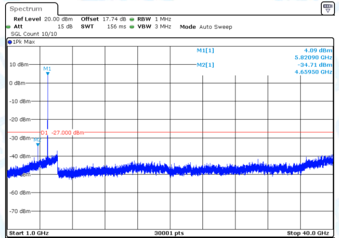
11N20SISO-Ant1-5785-1000~40000-PASS
