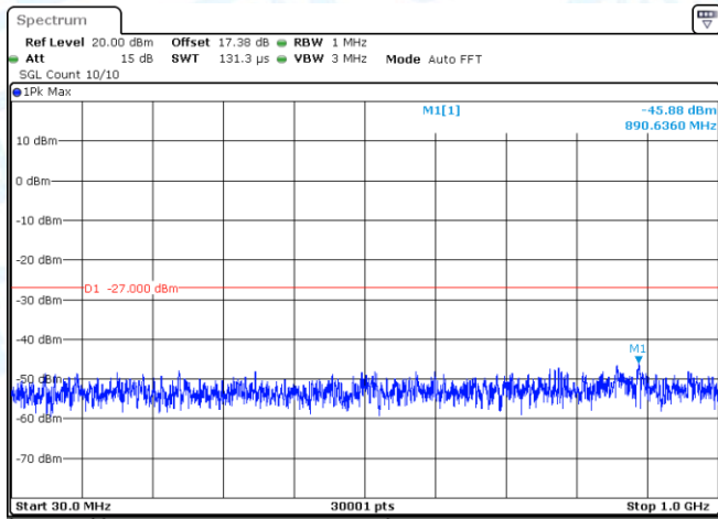
11AX20SISO-Ant1-5180-30~1000-PASS
