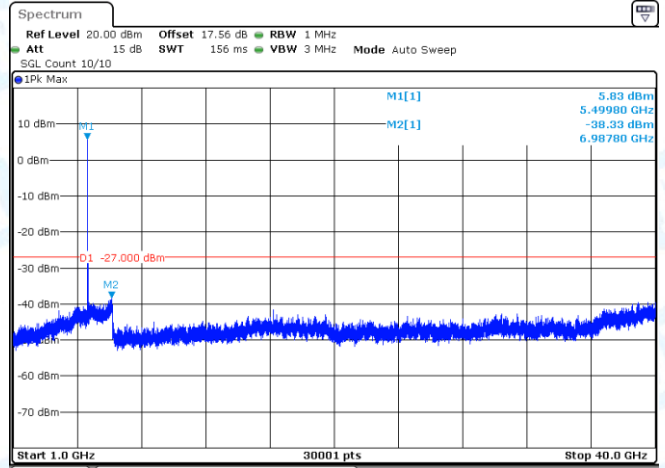
11AC20SISO-Ant1-5500-1000~40000-PASS
