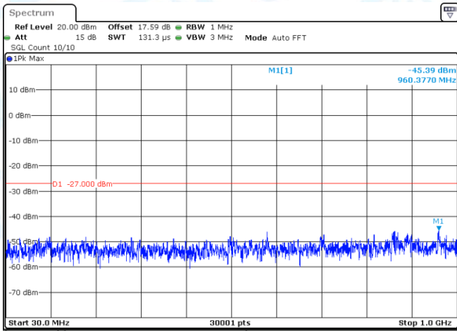
11N20SISO-Ant1-5500-30~1000-PASS
