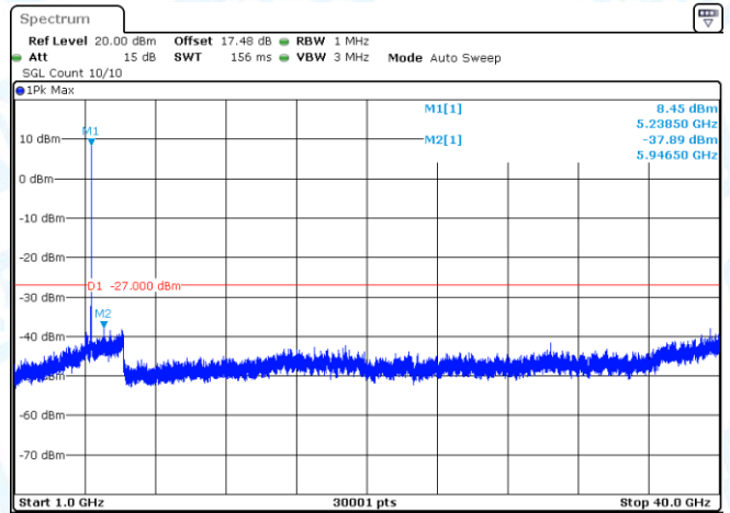
11AC20SISO-Ant1-5200-1000~40000-PASS
