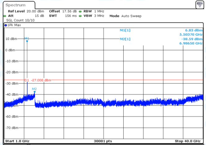
11A-Ant1-5500-1000~40000-PASS
