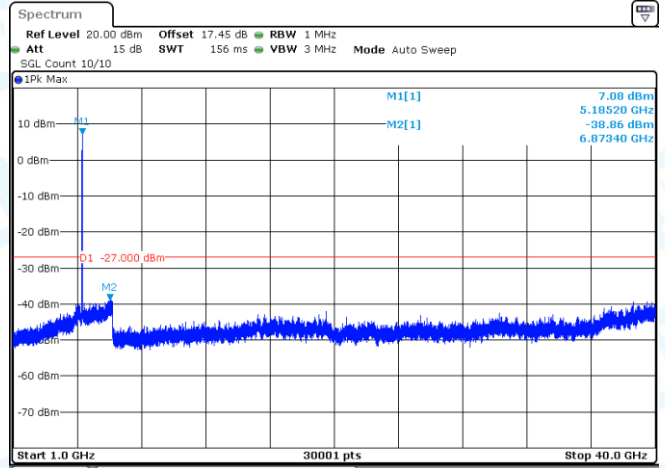
11AC20SISO-Ant1-5180-1000~40000-PASS
