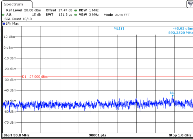
11N20SISO-Ant1-5260-30~1000-PASS
