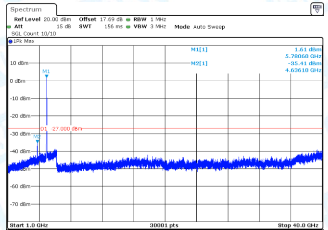
11AC40SISO-Ant1-5755-1000~40000-PASS
