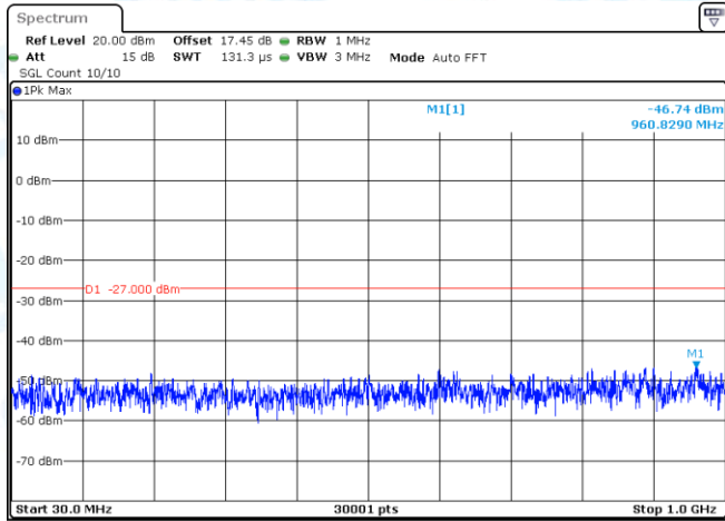
11AX20SISO-Ant1-5180-30~1000-PASS
