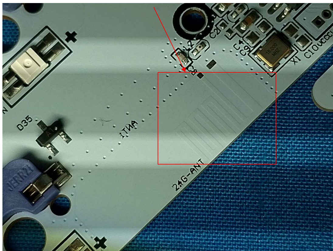
Bluetooth&SRD Antenna
