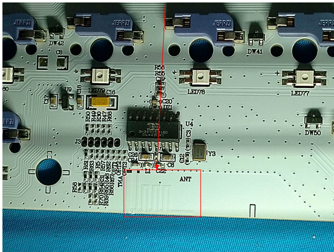
Bluetooth&SRD Antenna
