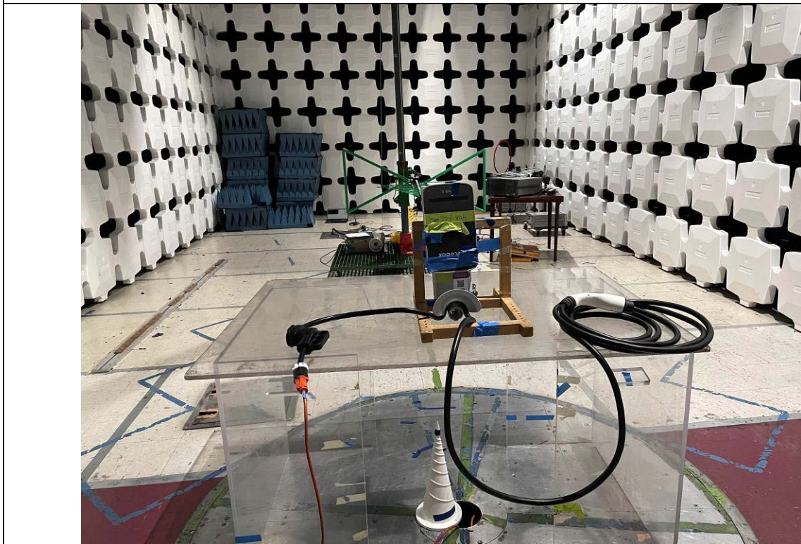
Radiated Emission Test below 1GHz Rear View
