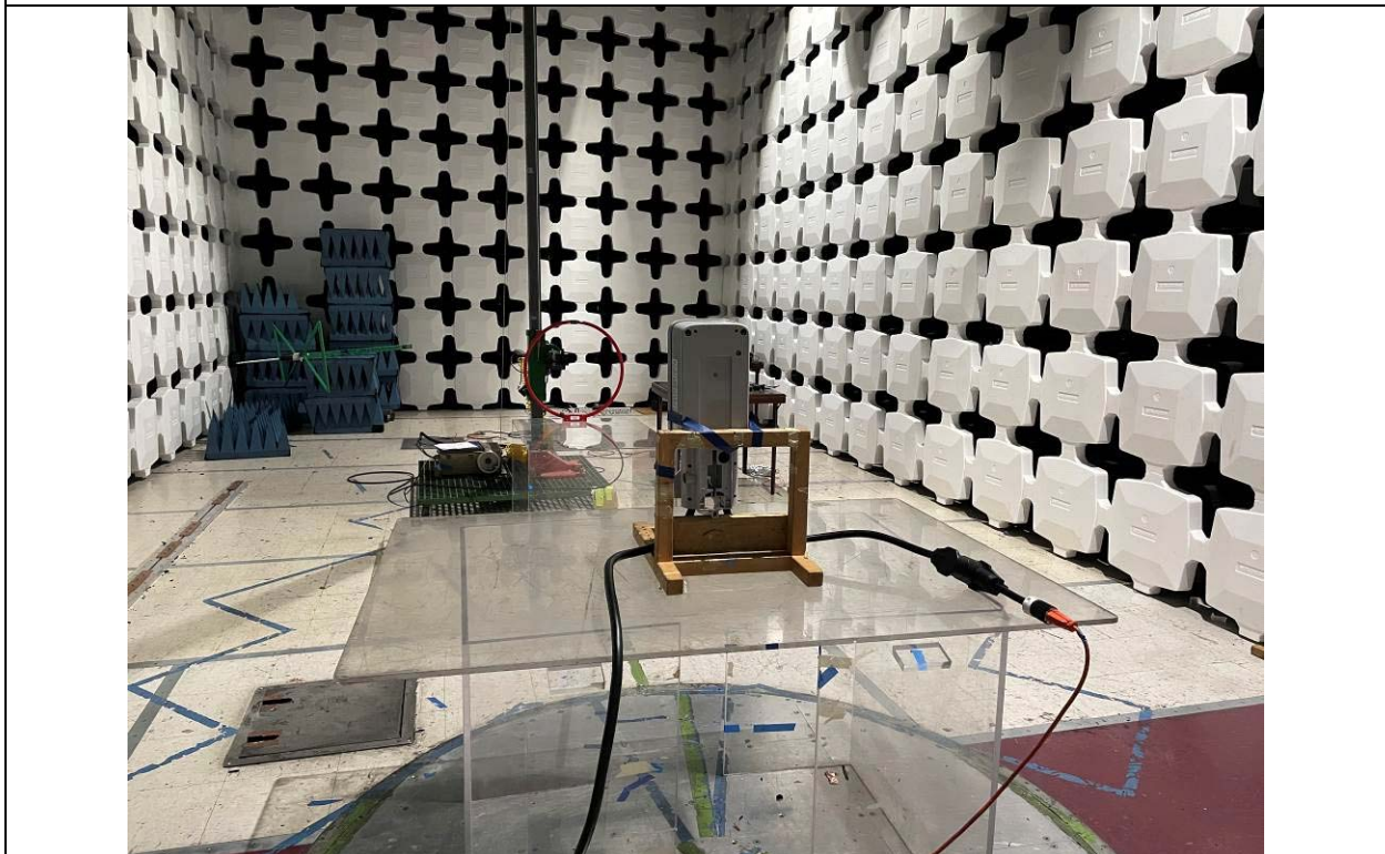
Radiated Emission Test below 30MHz Rear View
