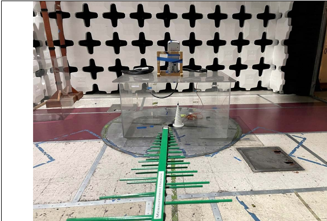
Radiated Emission Test below 1GHz Front View
