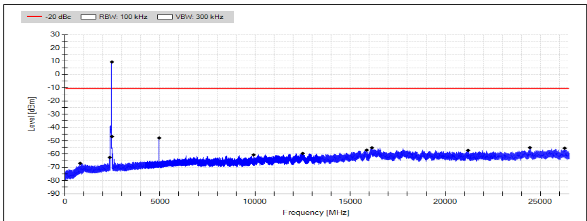
Figure 40: Conducted spurious emissions 30 - 26500 MHz channel 39, power setting 145, PHY 125k
