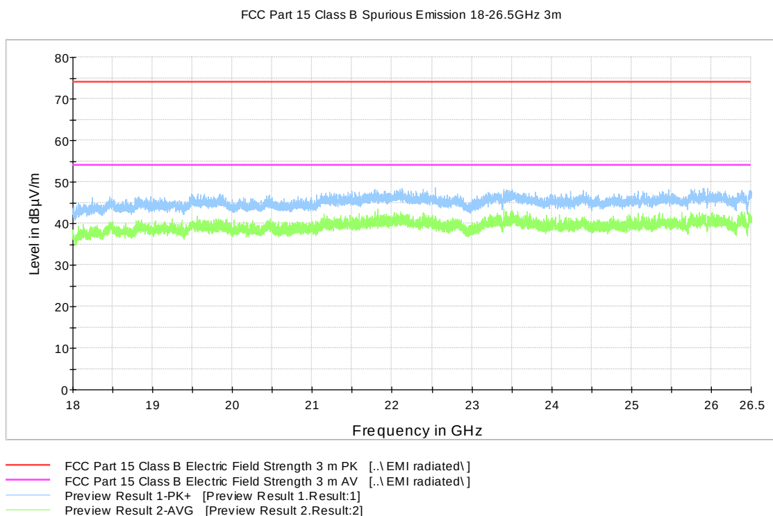
Figure 23: Channel 39 high 18 GHz – 26.5 GHz (A)
