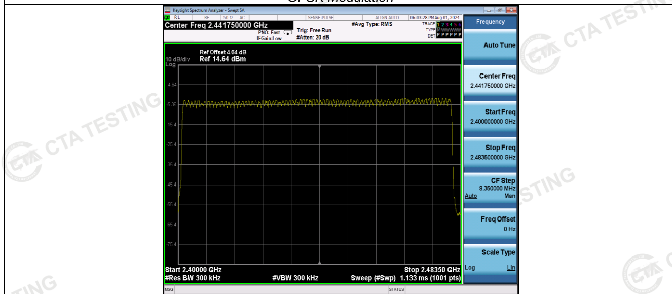
m/4DQPSK Modulation
