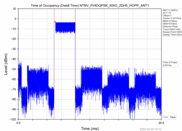
2DH5
