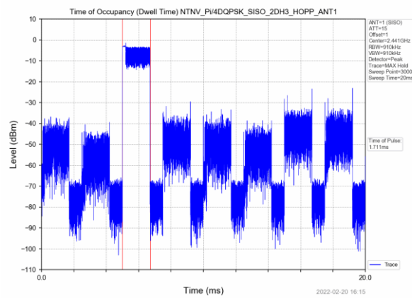
2DH3
