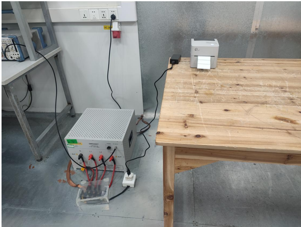
FCC ID: 2A4KS-2054K-WF Photo of Conducted Emission Test
