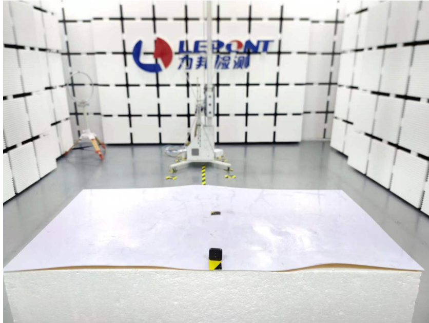
Radiated Emission
