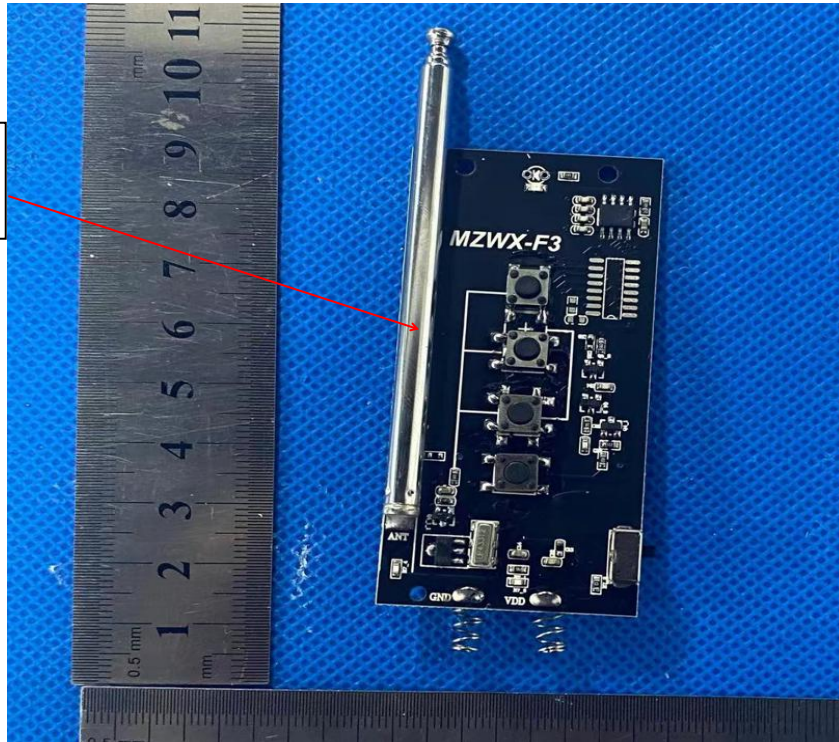
433.92MHz Antenna
