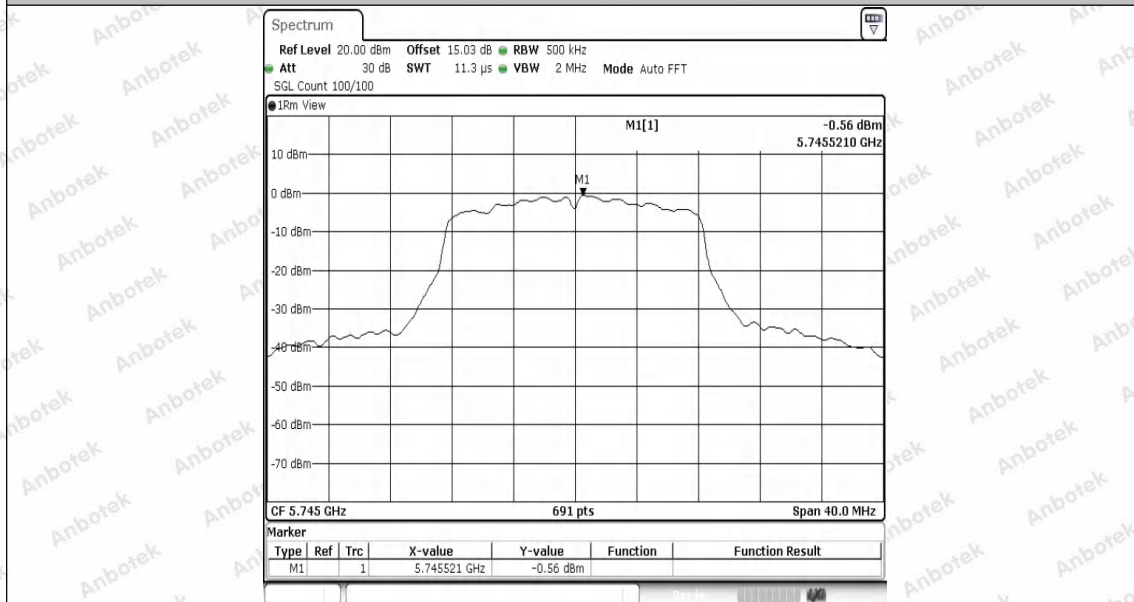
11A-Ant1-5745-PASS
