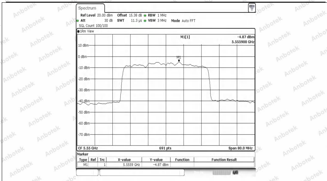
11AX40SISO-Ant1-5550-PASS
