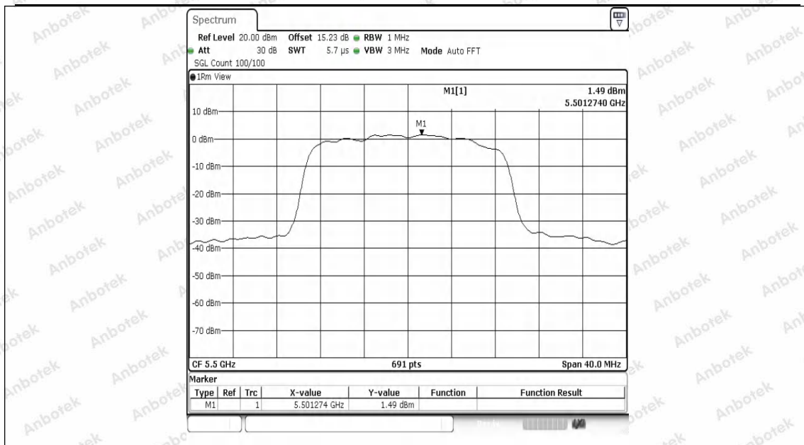
11N20SISO-Ant1-5500-PASS
