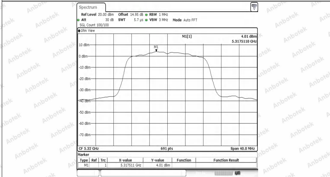
11N20SISO-Ant1-5320-PASS
